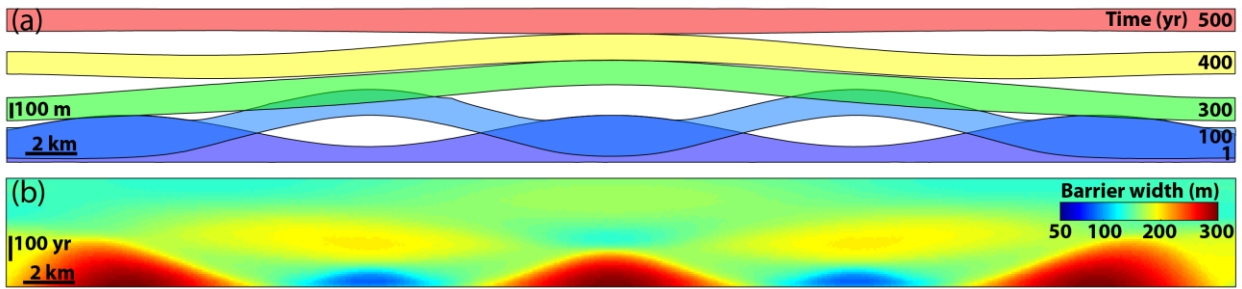
Figure 5. BRIE without inlets showing barrier response to variations in the initial back-barrier position x_b (see also Ashton and Lorenzo-Trueba, 2018), (a) x_s and x_b at 5 instances, (b) barrier width as a function of time. Minima in barrier width drive faster transgression, which in turn results in wider barriers through accumulation of alongshore sediment.
