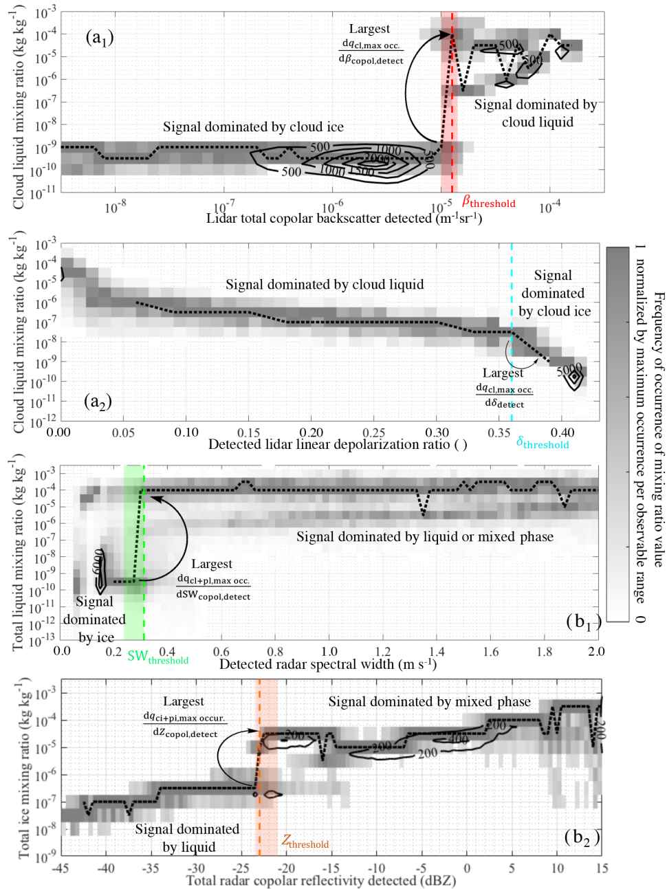
Figure 6. Example of joint frequency of occurrence histograms (contours) and normalized subsets from the joint histograms (gray shading) for one (GO) 2 -SIM forward realization: (a 1 ) \beta_{\text{copol,total,detect}} , (a 2 ) \delta_{\text{detect}} , (b 1 ) SW_{\text{copol,detect}} , and (b 2 ) Z_{\text{copol,total,detect}} . These are used for the determination of objective water-phase classifier thresholds (vertical colored dashed lines) that are set at the observational value with the largest change (see curved arrows) in most frequently occurring mixing ratio. These thresholds are not fixed but rather reestimated for each forward-ensemble member. The widths of the color-shaded vertical columns represent the interquartile range spreads generated from 576 different forward realizations.
