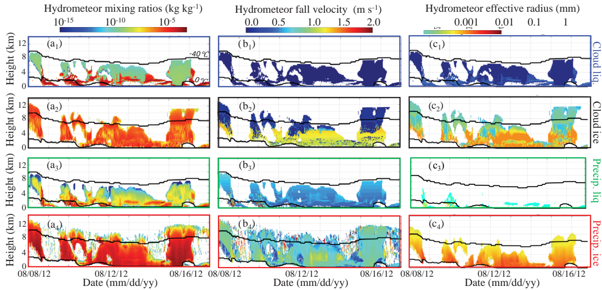
Figure 2. Sample time series of ModelE outputs: (a 1–4 ) mixing ratios, (b 1–4 ) mass-weighted fall speed (positive values indicate downward motion) and (c 1–4 ) effective radii for cloud droplets (1; blue boxes), cloud ice particles (2; black boxes), precipitating liquid drops (3; green boxes), and precipitating ice particles (4; red boxes). Also indicated are the locations of the 0 and -40^{\circ}\text{C} isotherms (horizontal black lines).
