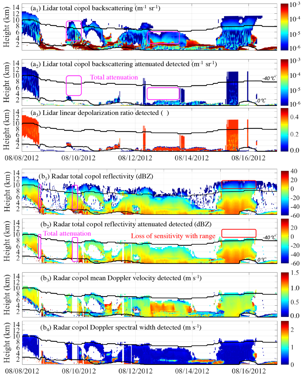
Figure 4. Example outputs from the (GO) 2 -SIM backscattered power modules (1), sensor capability modules (2), and specialized-observables modules (3–4) for (a) lidars and (b) radars obtained using one set of empirical backscattered power relationships. This figure highlights sensor limitations ranging from attenuation (magenta boxes) to sensitivity loss with range (red boxes). Also indicated are the locations of the 0 and -40^{\circ}\text{C} isotherms (black lines). Note that positive velocities indicate downward motion.
