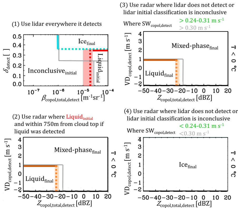
Figure 7. Collective illustration of hydrometeor-phase classification thresholds and phase-classification sequence. Fixed empirical thresholds modified from Shupe (2007) are displayed as gray lines. The objectively determined flexible thresholds are displayed using dashed colored lines and colored shading as in Fig. 6. Note that positive velocities indicate downward motion.
