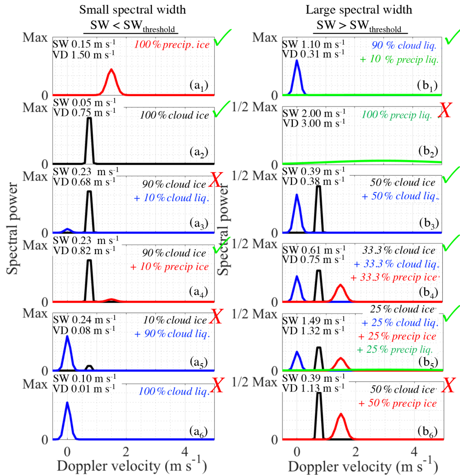
Figure 5. Cartoon examples of radar Doppler spectra from different hydrometeor combinations: precipitating ice (red), cloud ice (black), precipitating water (green), and cloud water (blue). The contribution of each hydrometeor species to the total copolar reflectivity is indicated in the top right of each subpanel. Each radar Doppler spectrum has been normalized to have the same total copolar radar reflectivity, which highlights the fact that different hydrometeor combinations generate unique mean Doppler velocity (VD) and Doppler spectral width (SW) signatures. As discussed in Sect. 6, low spectral width signatures are assumed to be associated with ice conditions (column a), while high spectral width signatures are assumed to be associated with liquid–mixed-phase conditions (column b). Hydrometeor combinations that respect these assumptions are marked with ✓ marks. Exceptions to these rules (X marks) are responsible for (GO) 2 -SIM phase misclassifications above the level of lidar extinction. This list is not exhaustive.
