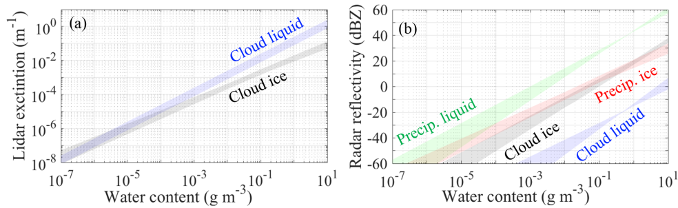
Figure 3. Relationship between water content in the form of cloud liquid (blue), precipitating liquid (green), cloud ice (black) and precipitating ice (red) and (a) lidar extinction, and (b) radar copolar reflectivity. Spread emerges from using multiple differing empirical relationships (listed in Table 2) and from variability in the 1-year ModelE output (including the effects of varying temperature and effective radii).
