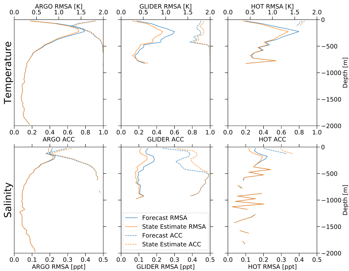
Figure 11. RMSA (solid) and ACC (dashed) profiles of subsurface temperature (top) and salinity (bottom) for Argo floats, SeaGliders and HOT CTDs for the forecast (blue) and the state estimate (orange). Data were binned into 50 m intervals.
