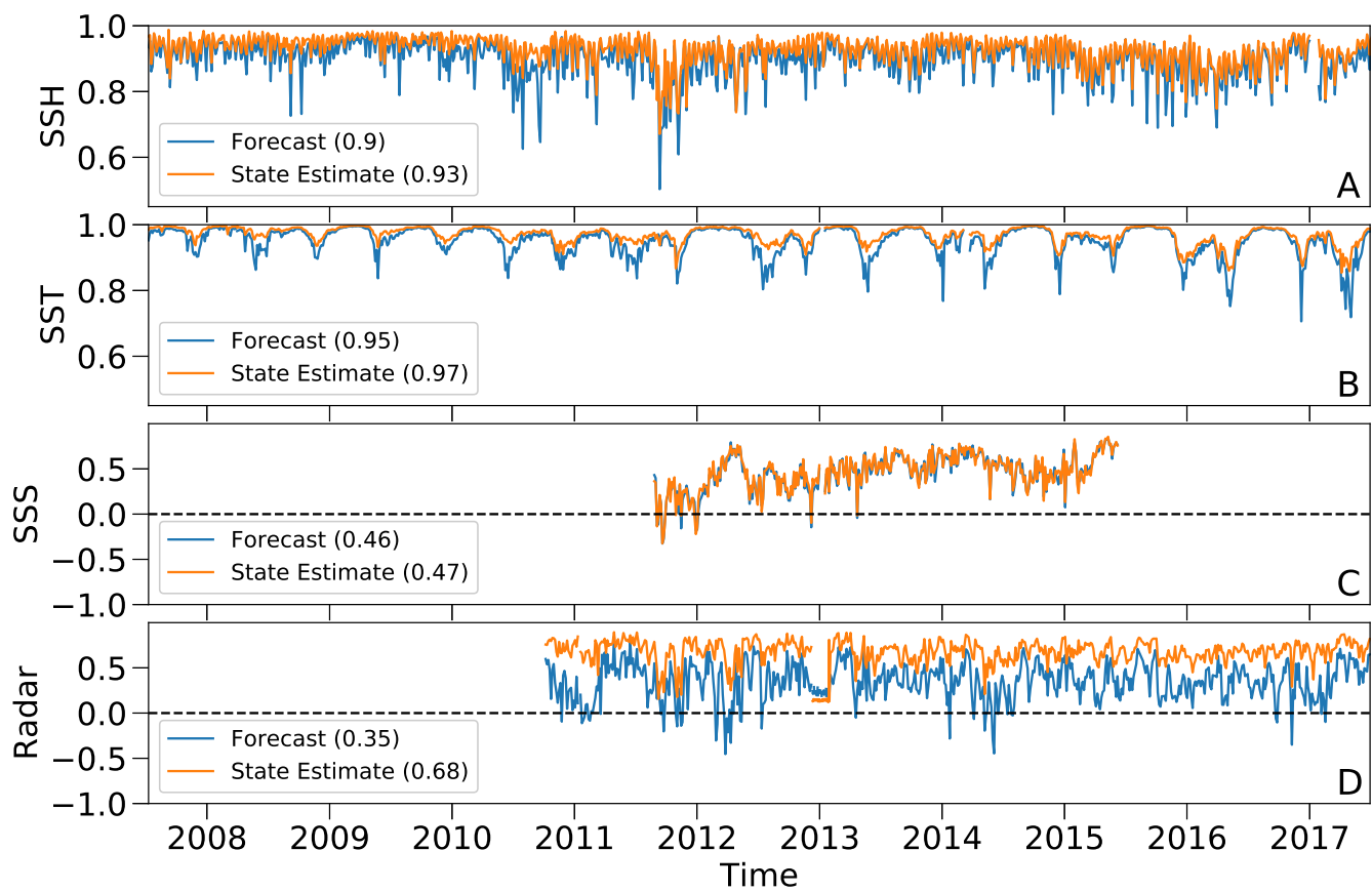
Figure 8. Time series of anomaly correlation coefficients (ACC) between remotely sensed observations and two model realizations; the state estimate (orange) and the forecast (blue). A) Sea Surface Height; B) Sea Surface Temperature; c) Sea Surface Salinity and D) HFRs
