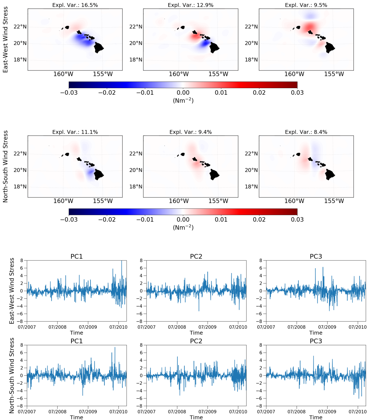
Figure 14. Spatial EOF patterns and principal components (PC) of wind stress perturbations for the period prior to the assimilation of HFR measurements (June 2007 - September 2010). The EOFs were calculated using the routines described in Dawson (2016).
