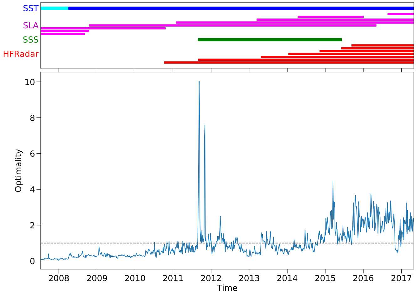
Figure 5. Top - Gantt chart of remotely sensed observations used in the study. Bottom - Optimality of I4D-Var data assimilation with the dashed line representing the theoretical minimum.
