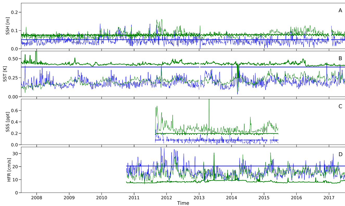
Figure 6. Time series of spatially averaged background (blue) and observation (green) errors, with thick lines showing a priori values and thin lines the posterior calculated using Equations (5) and (7). A) Sea Surface Height; B) Sea Surface Temperature; C) Sea Surface Salinity and D) HFR.
