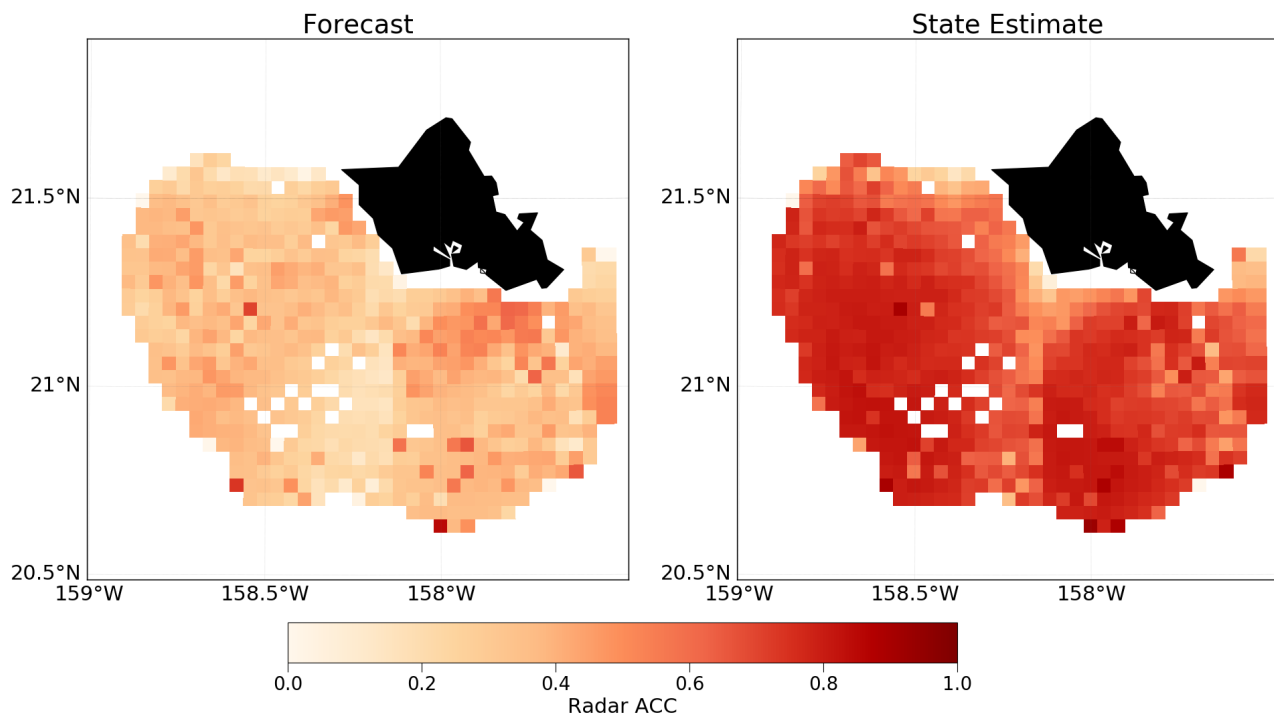
Figure 10. Spatial maps of HFR statistics for south O'ahu for the forecast (left) and the state estimate (right). Top panel: RMSA; bottom panel: ACC.
