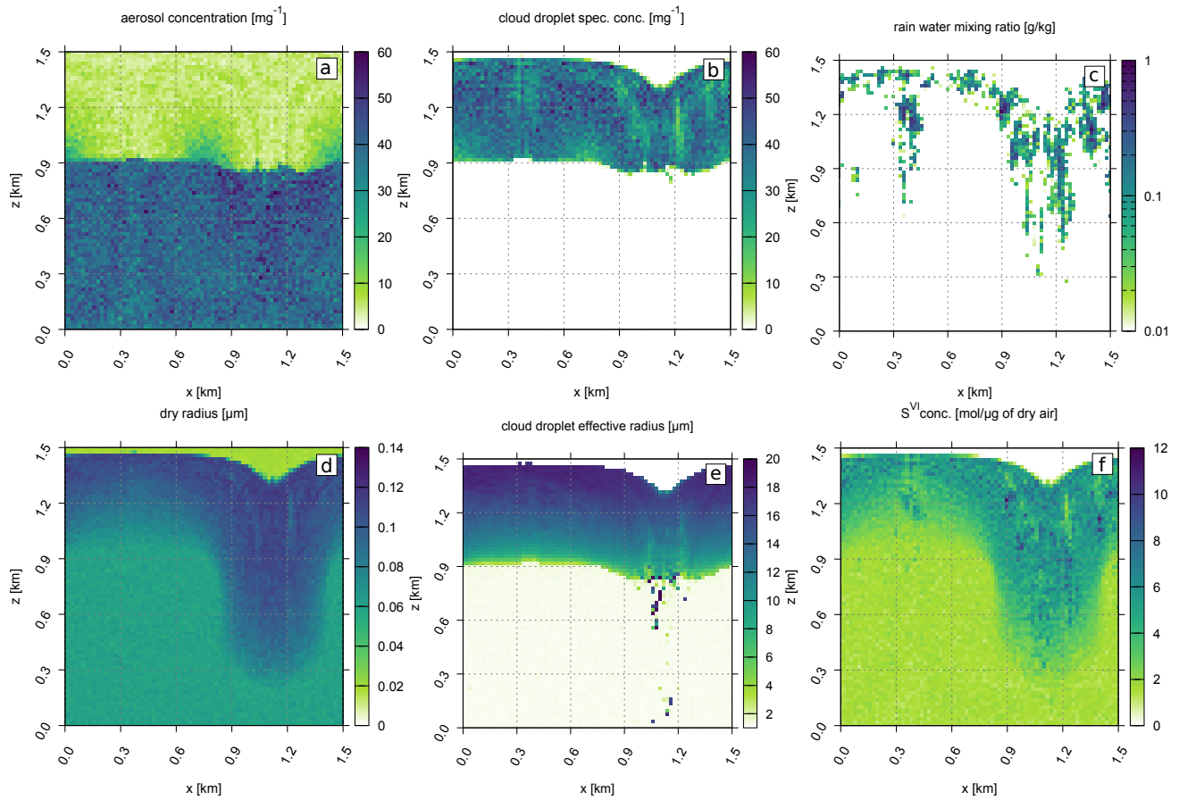
Figure 4. Base case setup (see Tab. 2). All panels depict model state after 30 minutes simulation time (excluding the spin-up) and show: unactivated aerosol concentration (a), cloud droplet specific concentration (b), rain water mixing ratio (c), mean dry radius (d), cloud droplet effective radius (e) and concentration of S VI molecules (f). The thresholds for particle radii are: unactivated aerosol < 1 \mu\text{m} ; 1 \mu\text{m} < \text{cloud} < 25 \mu\text{m} ; rain > 25 \mu\text{m} . Note the logarithmic scale for the rain water mixing ratio plot.
