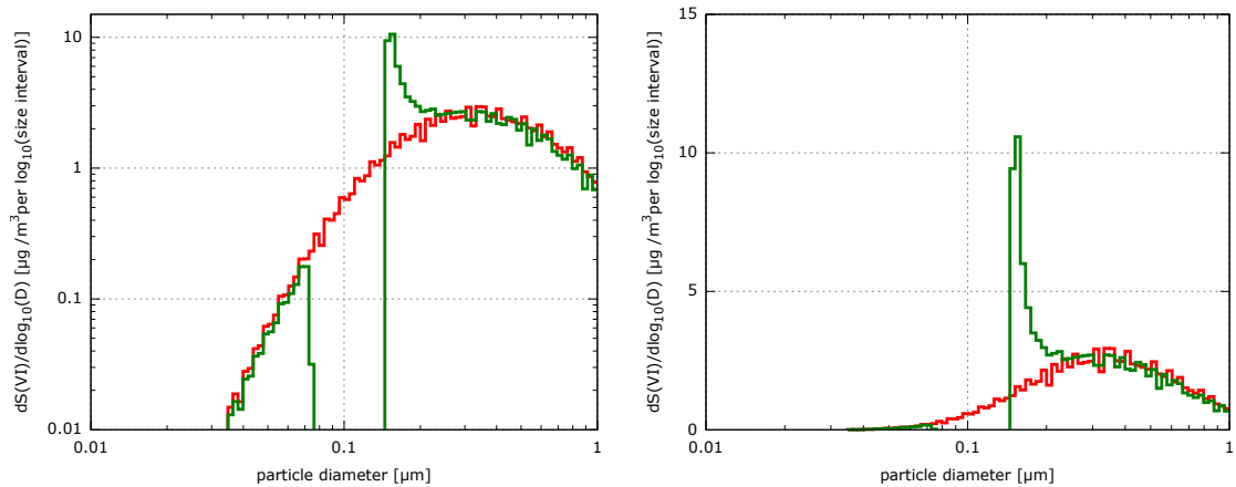
Figure 3. Modification of the dry aerosol sulfate mass. Red line shows the initial condition and green line shows the final model state. Left panel uses logarithmic ordinate and right panel uses linear ordinate.
