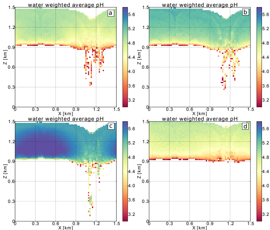
Figure 5. Liquid water volume weighted average pH from base case (a), case1 (b), case2 (c), case3 (d). See Tab. 2 and Tab. 3 for a definition of simulation setups.
