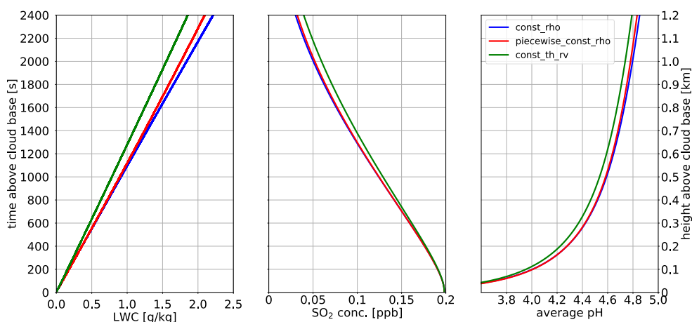
Figure 1: The parcel model simulations using three different ways to calculate the pressure and dry air density profiles: assuming constant density profile (blue), assuming piecewise constant density profile (red) and assuming constant potential temperature and water vapor mixing ratio profile (green). The panels show the liquid water mixing ratio, the \text{SO}_2 concentration and the water volume weighted average pH, respectively.
