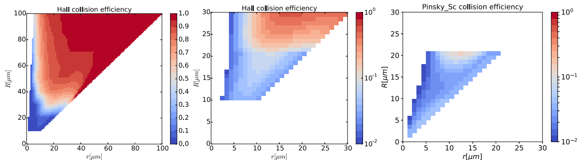
Figure 2: The collision efficiencies used in the presented simulations. The left panel shows the Hall (1980) collision efficiency. The middle panel zooms-in to show the Hall (1980) collision efficiency for small droplets. The right panel shows the collision efficiency for small droplets based on Pinsky et al. (2008).
