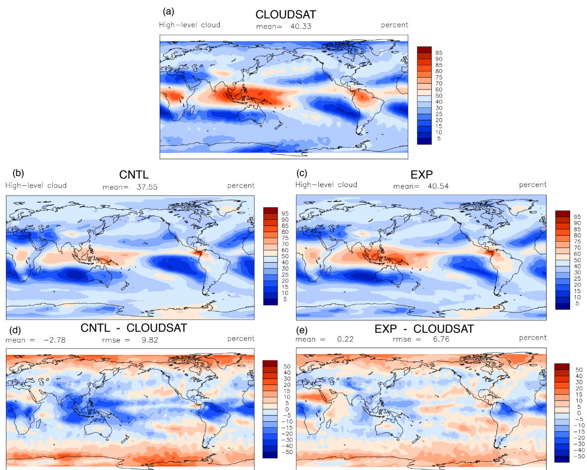
Figure 4. The spatial distribution of high cloud amount in (a) observation, (b) CNTL, (c) EXP, (d) CNTL minus observation, (e) EXP minus observation.
