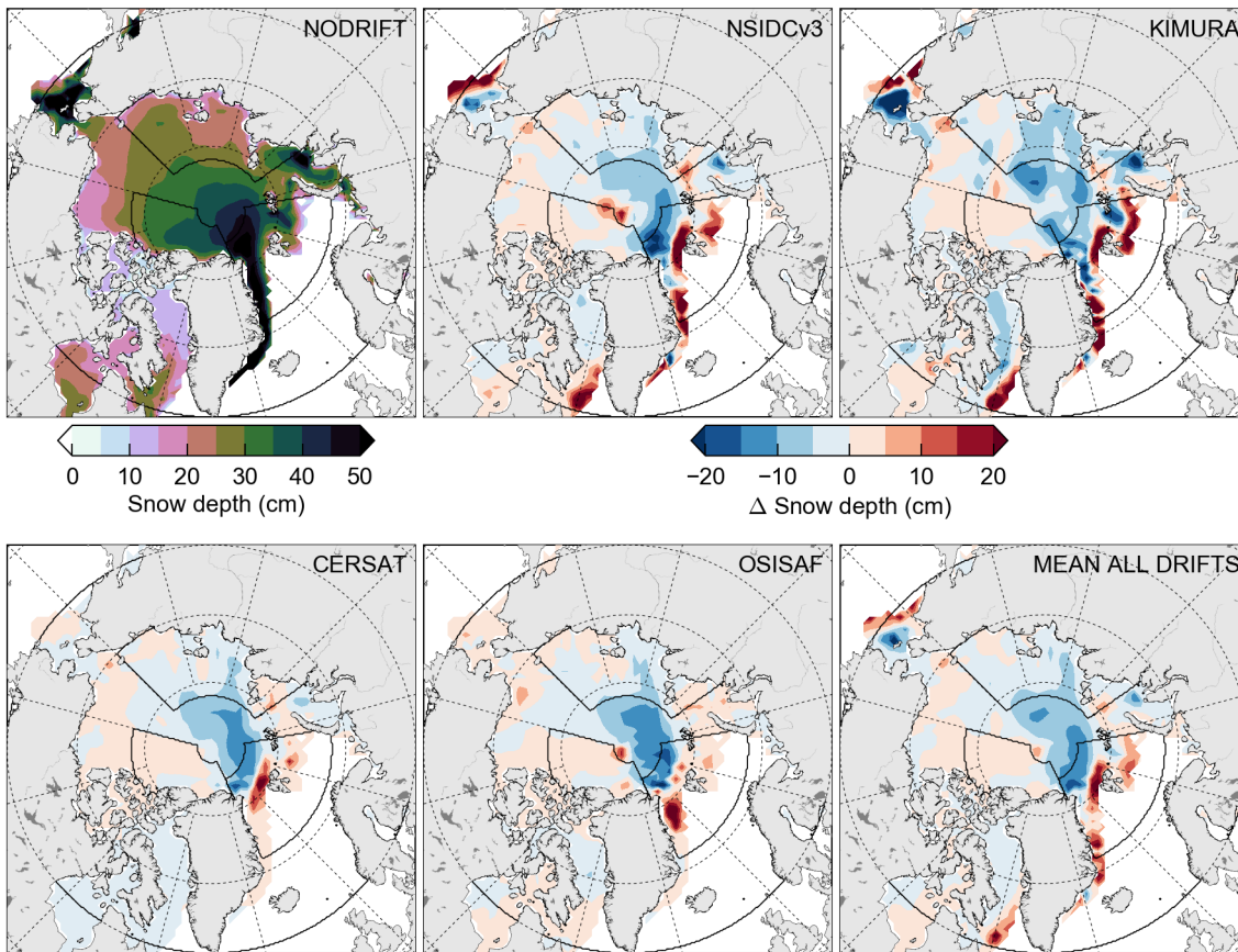
Figure 12: Modeled snow depth on May 1st (averaged over May 1 st 2011, 2013, 2014, 2015), assuming no ice motion (NODRIFT, top left) and then the difference to the simulations forced by the four different ice motion products and the mean snow depth from the four different forced model runs.
