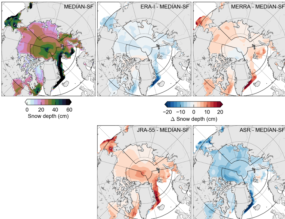
5 Figure 10: Simulated snow depths on May 1st (averaged over May 1 st 2001 to 2015), using the MEDIAN-SF snowfall forcing (top left) and then the difference to the simulations forced by the four different snowfall products (bottom and top right). The ASRv1 forced results are limited to May 1st 2012. Red (blue) colours indicate the individual reanalysis-forced simulations have higher (lower) snow depth.
