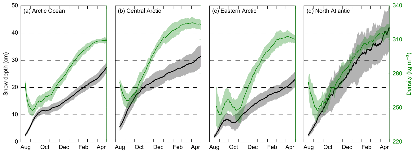
5 Figure 6: Seasonal snow depth (black) and bulk density (green) evolution across the four study regions (shown in Figure 5) initiated from August 15 th 2000-2014 and run until May 1 st of the following year using the MEDIAN-SF/parameter settings (Table 1). The thick lines show the mean values over this time period, while the shaded areas represent the interannual variability (one standard deviation).
