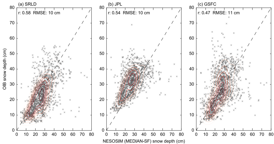
5 Figure 15: Scatter plots of NASA’s Operation IceBridge (OIB) snow depths from the three OIB products binned onto our 100 km model grid, and coincident NESOSIM/MEDIAN-SF snow depth estimates for all years of data from 2009-2015, including the correlation coefficient ( r ) and root mean squared error (RMSE). The contours show the kernel density estimate of the distributions.
