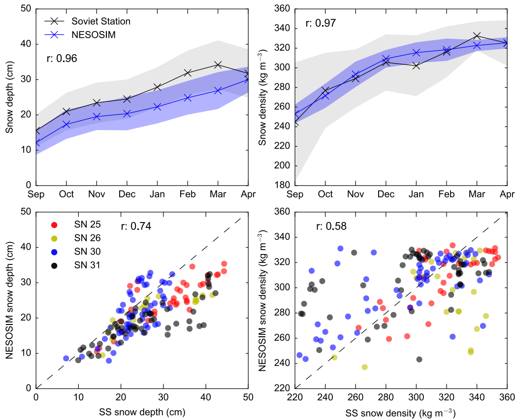
5 Figure 3: Comparison of NESOSIM snow depth (left) and snow density (right) data with drifting Soviet station data collected between 1981 and 1991. The top panels show the mean seasonal evolution of the snow depth and density for the model (blue) and Soviet station data (black), with the data binned into the different months the data were collected. The shaded area represents one standard deviation from the annual monthly mean. The bottom panels show scatter plots of all points for which there were temporal crossovers. The r-values indicate the correlation coefficient, while the colors indicate the different stations that collected the data. The NESOSIM data are from the default/ERA-I model configuration. 10
