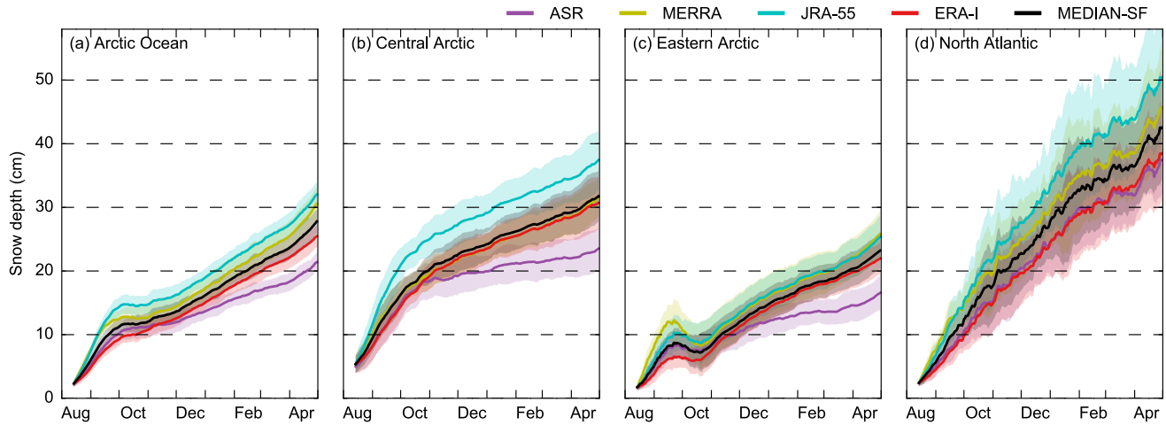
5 Figure 9: Seasonal snow depth evolution across the four study regions (shown in Figure 5) initiated from August 15 th 2000-2014 and run until May 1st of the following year, forced by five different reanalysis snowfall products. This figure also includes results using the ASRv1 forced simulations (which are limited to Aug 15th 2000 to May 1st 2012). The thick lines show the mean (daily) regional snow depths over this time period, while the shaded areas represent interannual variability (one standard deviation). All model runs use the default forcings/parameter settings. 10
