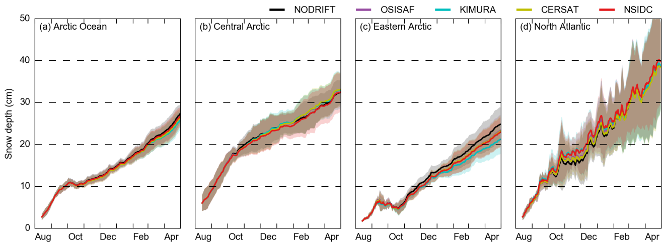
Figure 11: Seasonal snow depth evolution across the four study regions (shown in Figure 5), initiated in August 15 th 2010, 2012, 2013, 2014 and run until May 1st of the following year, forced by four different ice motion datasets and assuming no ice motion (NODRIFT). The thick lines show the mean (daily) regional snow depths over this time period, while the shaded areas represent interannual variability (one standard deviation). All model runs use the default/MEDIAN-SF parameter settings.
