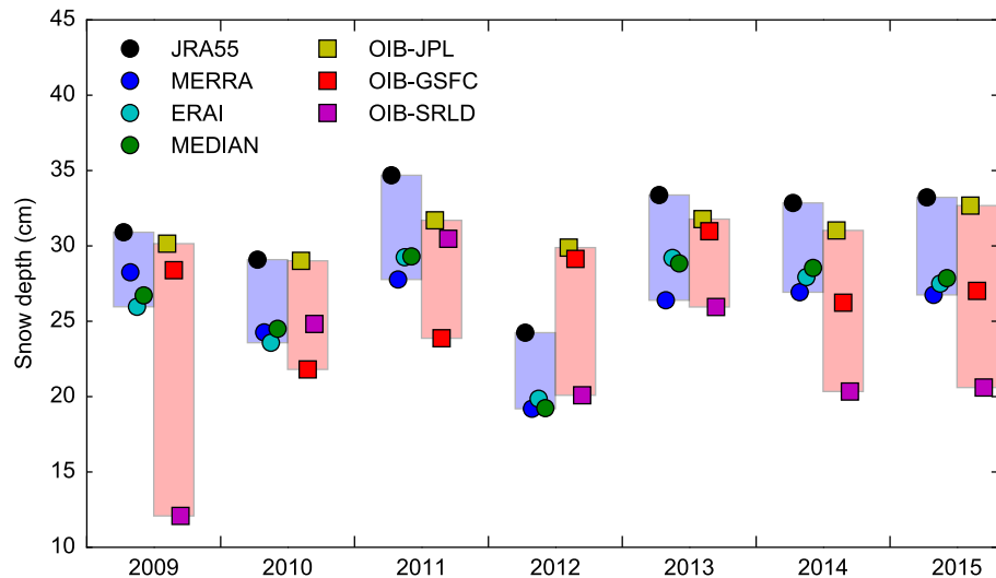
5 Figure 14: Comparisons of the annual mean snow depths from NESOSIM (default configuration) forced with different reanalyses, and the various Operation IceBridge (OIB) snow depth products. The blue (red) shading represents the annual mean spread across the different NESOSIM results (OIB products). The markers are spread across the shaded areas to improve readability.
