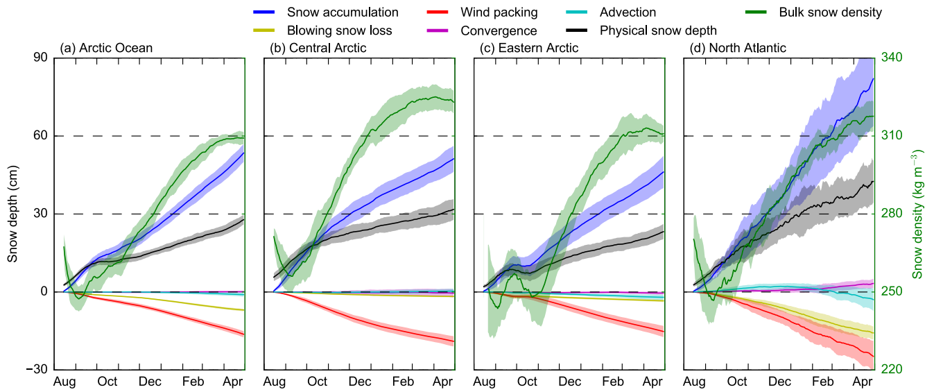
Figure 7: Seasonal snow budget evolution across the four study regions (shown in Figure 5), initiated from August 15 th 2000-2014 and run until May 1st of the following year using the default/MEDIAN-SF NESOSIM simulations. The thick lines show the mean, daily, regional values over this time period, while the shaded areas represent the interannual variability (one standard deviation).
