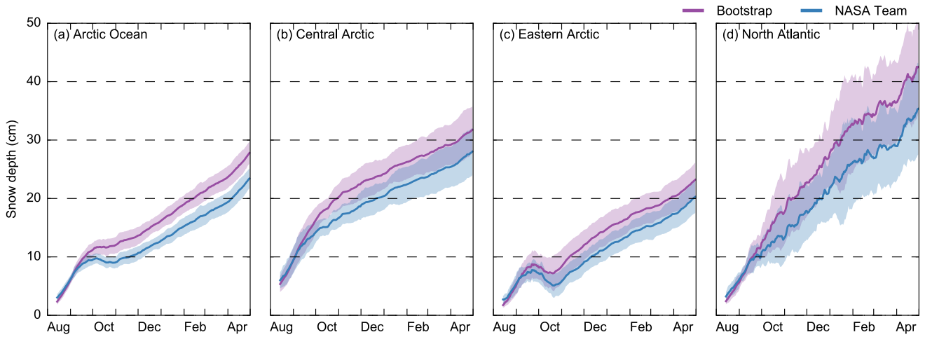
Figure 13: Seasonal snow depth evolution across the four study regions (shown in Figure 5), initiated from August 15 th 2000-2014 and run until May 1st of the following year, forced by the Bootstrap (magenta) and NASA Team (blue) ice concentration datasets. The thick lines show the mean (daily) regional snow depths over this time period, while the shaded areas represent interannual variability (one standard deviation). All model runs use the default/MEDIAN-SF configuration.
