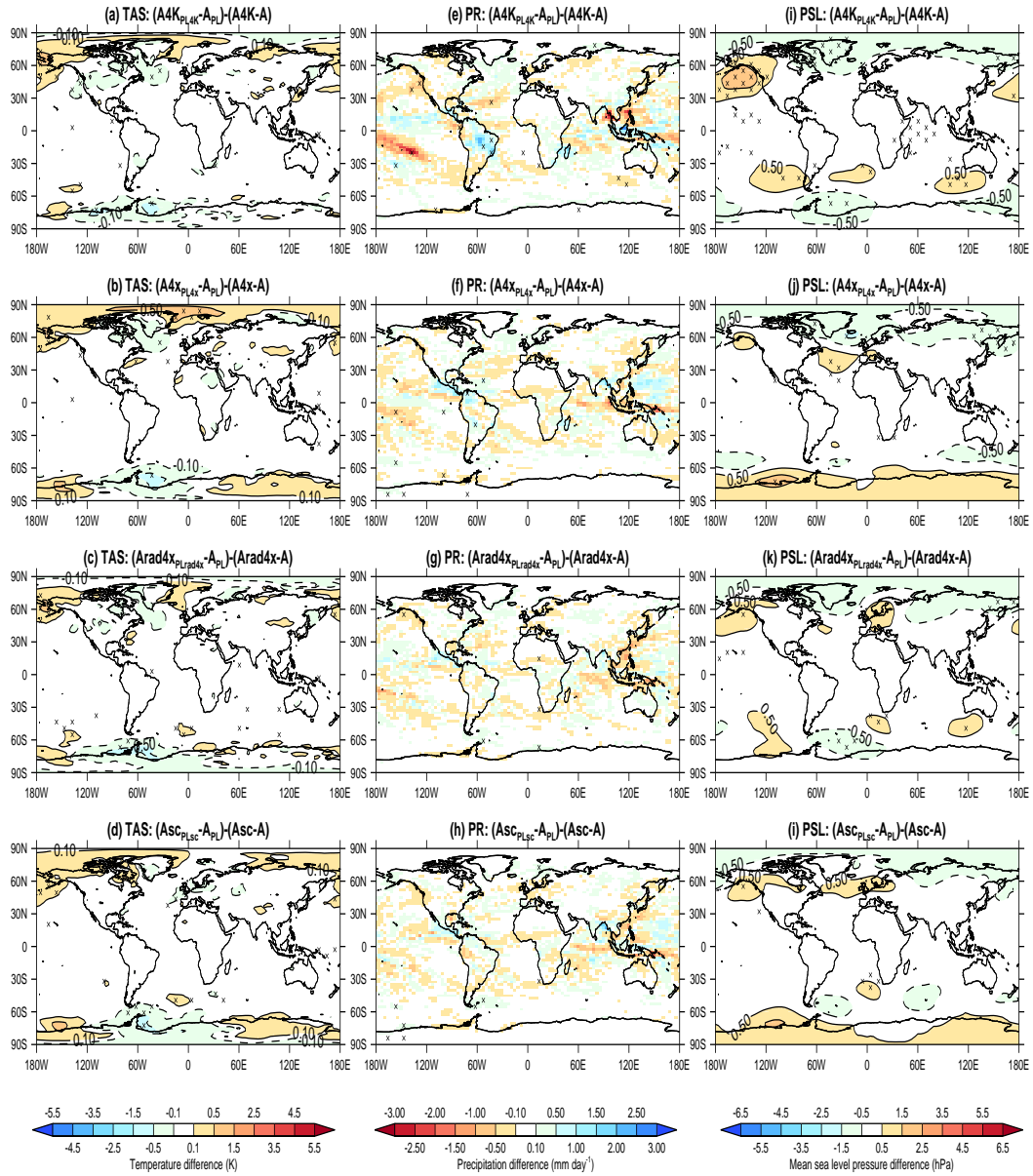
Figure 2. Differences in surface air temperature (TAS, K) for (a) [A4K PLAK -A PL ]-[A4K-A] (b) [A4x PL4x -A PL ]-[A4x-A], (c) [Arad4x PLrad4x -A PL ]-[Arad4x-A] and (d) [Asc PLsc -A PL ]-[Asc-A]. Equivalent differences between simulations are given in (e)–(h) and (i)–(l) for precipitation (PR, mm day -1 ) and mean sea level pressure (PSL, hPa), respectively. The points labelled with an "x" indicate the differences are statistically significant using the Student's t-test ( p \leq 0.05 ).
