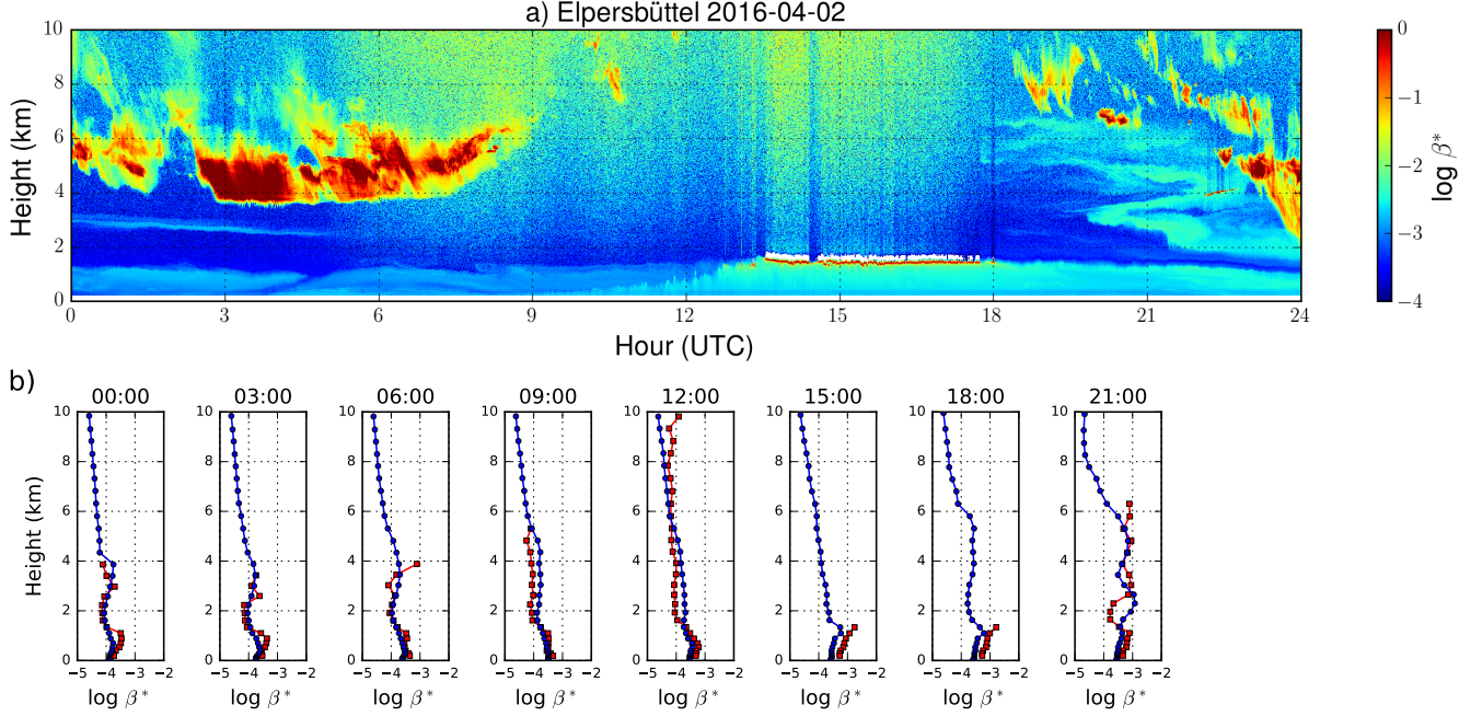
Figure 10. Time series of attenuated backscatter measured by the ceilometer at Elpersbüttel during a dust episode on 2 April 2016 is shown in (a). Attenuated backscatter calculated from model simulations (blue curve) is shown in (b), ceilometer measurements (red curve) are averaged to model resolution and shown for reference.
