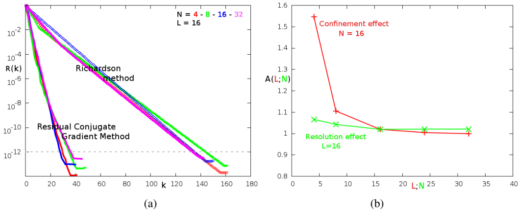
Figure 9. Potential flow around a cylinder: (a) Velocity convergence of two iterative methods (Residual Conjugate Gradient, Richardson) for different spatial resolutions N = [4 : 32] ( L = 16 ); (b) Evolution of the added mass coefficient A(N; L) with the confinement L = L_{cyl}/R_{cyl} ( N = 16 ) and with the nodes number per radius cylinder N ( L = 16 ). The confinement is defined in Fig. 9-a.
