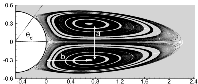
Figure 12. Recirculating region at Re = 40 (MNH-IBM, 20pts/D_{cyl} ): definition of the \theta_d ( \check{r} ) separation angle, l_r recirculating length and ( a ; b ) vortex core location. The distance are dimensionless by D_{cyl} .
