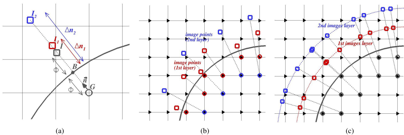
Figure 2. (a) Node definitions acting in the Ghost-Cell Technique : the ghost ( G ), interface ( B ), normal vector ( \vec{n} ), mirror ( I ) and images ( I_1, I_2 ). (b) resp. (c) Illustration of the classical (resp. new) GCT using the mirror (resp. images). Triangles correspond to one of the node types (see Fig. 1-b).
