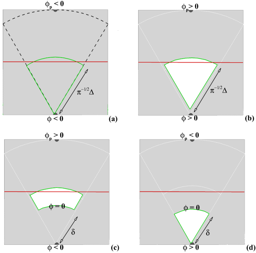
Figure 6. (a,b,c,d) \pm \widetilde{\Delta^2 \bar{u}_i^*} calculations depending on the signs of \phi_i = (\phi) and \phi_p on an arbitrary piece of cake. The white (resp. grey) region corresponds to the solid (resp. fluid) one of P_p^* (same colour code as in Fig. 5).
