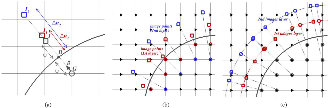
Figure 2. (a) Node definitions acting in the Ghost-Cell Technique : the G ghost ( G ), B interface ( B ), \mathbf{n} normal vector ( \mathbf{n} ), I mirror ( I ) and ( I_1, I_2 ) images ( I_1, I_2 ). (b) resp. (c) Illustration of the classical (resp. original/new ) GCT using the mirror (resp. images). Triangles correspond to one of the node types (see Fig. 1-b).
