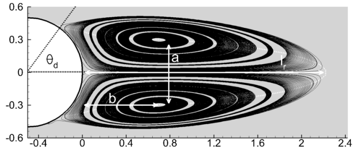
Figure 12. Recirculating region at Re = 40 (MNH-IBM, 20pts/D_{cyl} ): definition of the \theta_d (°) separation angle, l_r recirculating length and (a; b) vortex core location. The distance are dimensionless by D_{cyl} .
