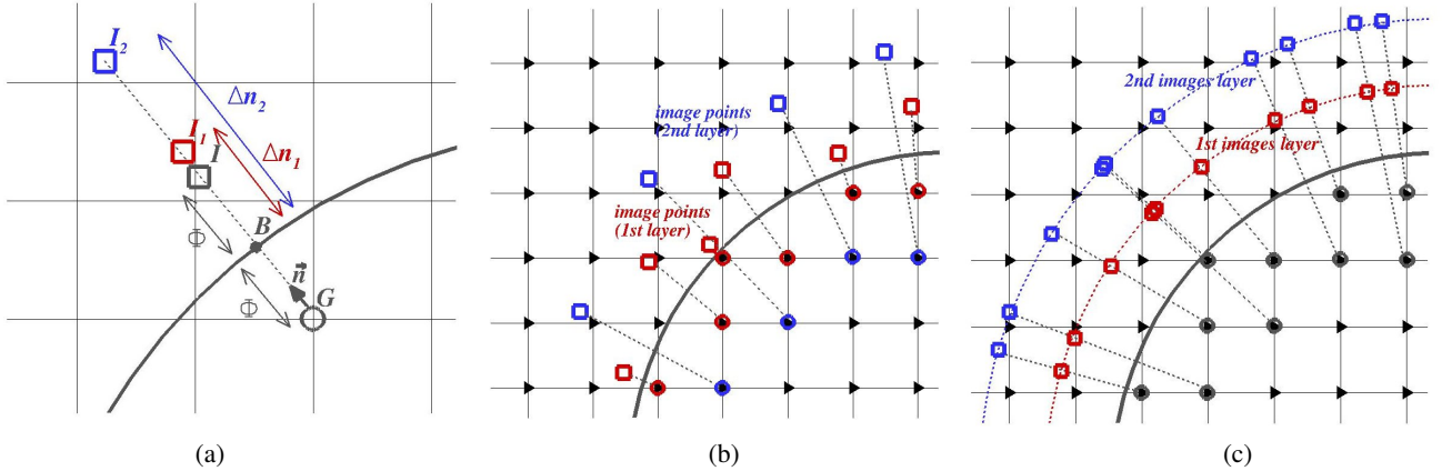
Figure 2. (a) Node definitions acting in the Ghost-Cell Technique : the G ghost , B interface , \mathbf{n} normal vector , I mirror and (I_1, I_2) images. (b resp. c) Illustration of the classical (resp. original) GCT using the mirror (resp. images). Triangles correspond to one of the node types (see Fig. 1-b).
