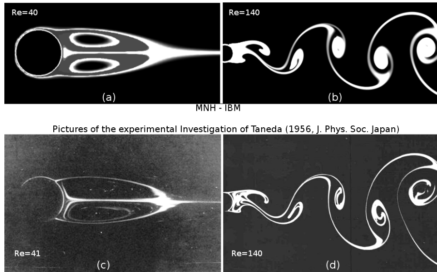
Figure 11. Eddies structure in a viscous fluid: Steady (left, Re \approx 40 ) and unsteady (right, Re \approx 140 ) solutions obtained by the current numerical investigation (top, MNH-IBM and 30pts/D_{cyl} ) and by the famous experimental Taneda (1956) investigation (bottom). The visualization is due to the presence of passive tracer injected on the body surface and transported by the flow.
