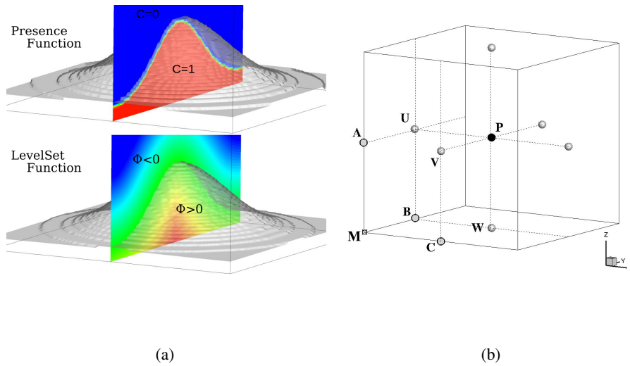
Figure 1. (a) Illustration of two ways to model a fluid-solid interface: the color code indicates the isocontours of the presence function C and the LevelSet function \phi Illustration of an interface separating fluid and solid regions; (b) Definition of the points type per cell: M the geometric/mesh point, P the mass point, U/V/W the velocity nodes and A/B/C the vorticity nodes.
