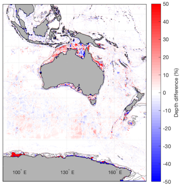
Fig. 1. Relative bathymetry change from OceanMAPS version 2.2.1 to version 3.0
