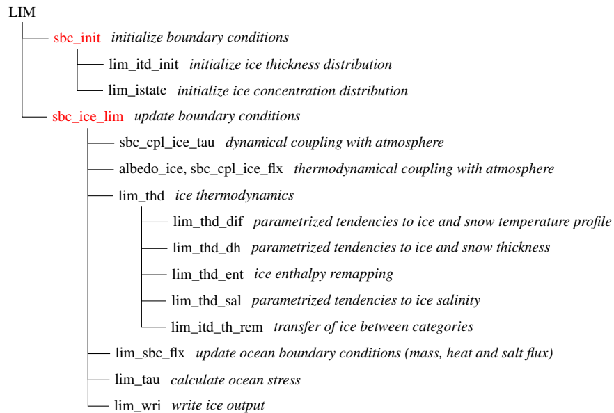
Figure 3. Flow-Simplified flow chart of the LIM model, part of the NEMO model if (nn_ice=3:LIM) in sbeice_lim (stp_cld) sea-ice is present. Routines dedicated to coupling via OASIS are coloured red.
