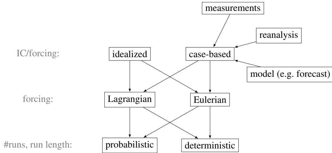
Figure 5. How Guideline on how to set up an SCM experiment. Each row represents a setup decision necessary (grey phrase on the far left) and potential approaches. IC is short for initial conditions.
