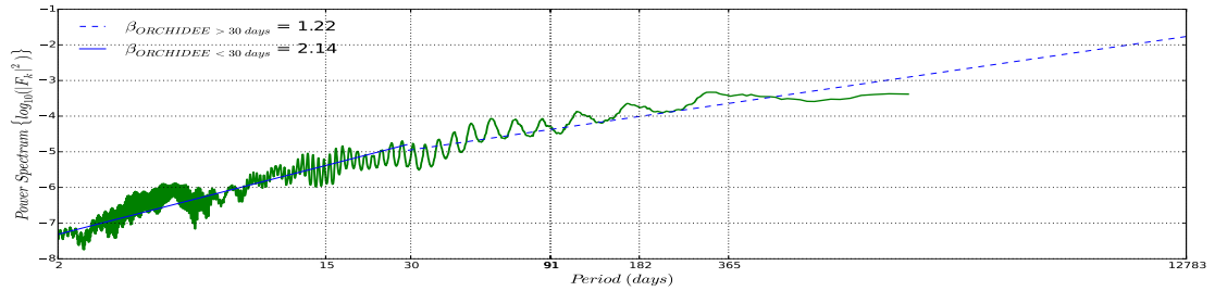
(b) Sub-surface runoff
