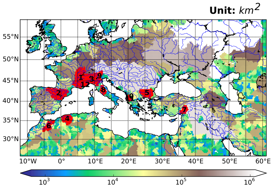
Figure 4. Extended simulation domain. The main watersheds are colored as a function of maximum upstream area ( km^2 ). They were extracted for an ORCHIDEE resolution of 1/4^\circ , with a threshold HTU number of 50. The twelve studied river basins are colored in red. They are numbered from 1 to 12, and the corresponding names are given in Table ???. The river network is plotted in blue based on the dataset from the Generic Mapping Tools ( http://gmt.soest.hawaii.edu ). River names are Rhône, Ebro, Po, Chelif, Maritsa, Moulouya, Ceyhan, Tiber, Adige, Shkumbinit, Devollit, Var corresponded to number from 1 to 12, respectively.
