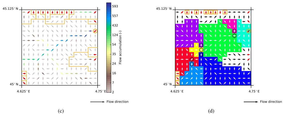
Figure 2. A schematic diagram of catchment construction in the revised-new river routing scheme of the ORCHIDEE land surface model (a) and illustration idea of Hydrological Transfer Unit (HTU): (b) Number of upstream HTUs contributing water to each grid box of the Rhône River at resolution of 1/8^\circ with a maximum number of HTUs per grid box of 9. Color is given in logarithm scale. Red rivers come from the Generic Mapping Tools dataset ( http://gmt.soest.hawaii.edu ). The small orange box shows the grid box of (c) and (d). (c) The orange ORCHIDEE grid box in (b) with information derived from HydroSHEDS at the 30 arc-second resolution: arrows show the flow direction of each HydroSHEDS pixel; brown to blue colors show flow accumulation; bold red arrows show the flow direction of the grid box outlets; the orange lines delineate the boundary of the preliminary HTUs; and the orange circle highlights the outlet points of the largest preliminary HTU in this grid box. (d) Partitioning of HTUs which share the same grid box outlet (marked by the orange circle). Hexagons denote the outlets of inter-HTUs based on the Pfafstetter codification and shaded color indicate the different HTUs. Flow direction arrows are displayed in black and white. Orange squares highlight the approximate 1 \text{ km}^2 HTUs.
