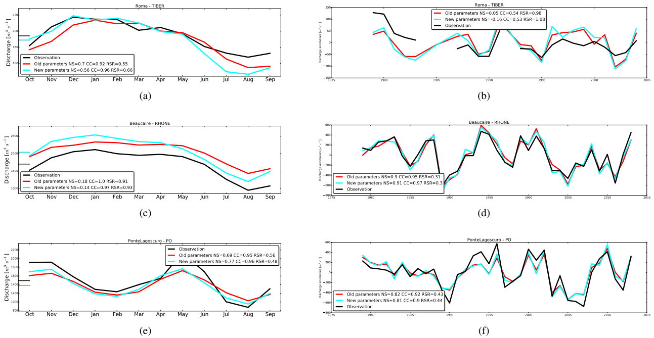
Figure 1. Mean annual cycle of river discharge (left column) and discharge anomalies (right column) during period of 1979-2013 simulated by the new RRS with old reservoir parameters (red line) and new reservoir parameters (cyan line), in comparison with observation (black line). Three station are investigated, includes Roma - the Tiber river (top panel), Beaucaire - the Rhone river (middle panel) and Pontelagoscuro - the Po river (bottom panel). Validation metrics are shown in legend boxes includes: NS - Nash-Sutcliffe coefficient, CC - the Pearson correlation coefficient (CC), RSR - the ratio of the Root Mean Square Error to the observation standard deviation.
