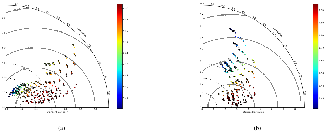
Figure 3. Taylor diagram investigates the sensitivity of simulated discharge to the varying reservoir parameters based on a theoretical test at the station Beaucaire, the Rhone river (a) and station Pontelagoscuro, the Po river (b). The color shows the Pearson correlation coefficient of simulated discharge between old and new routing scheme in corresponding to the experiments in Figure 2. The black star in the Taylor diagram denotes the result from the old routing scheme. The gray arcs are the axis for root mean square error.
