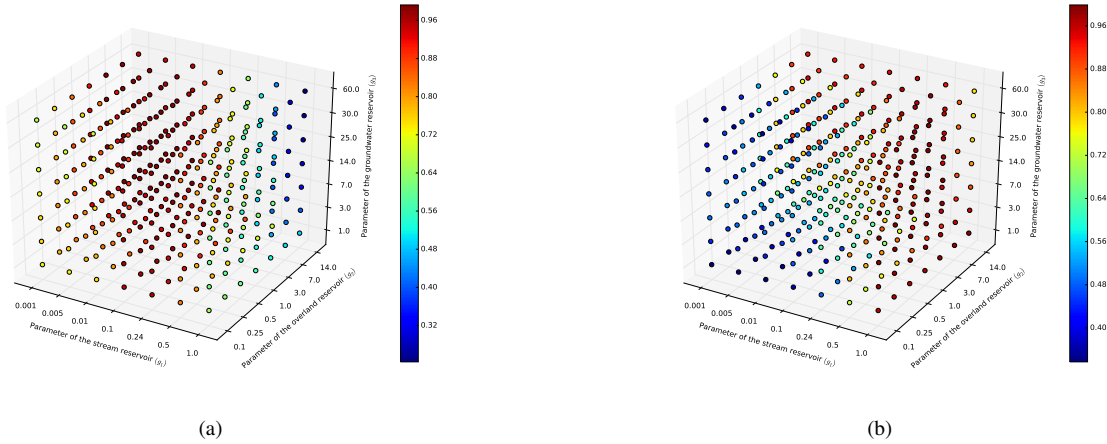
Figure 2. Sensitivity of simulated discharge to the varying reservoir parameters based on a theoretical test at the station Beaucaire, the Rhone river (a) and station Pontelagoscuro, the Po river (b). The color shows the Pearson correlation coefficient of simulated discharge between old and new routing scheme.
