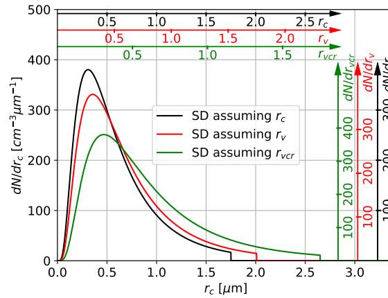
Figure 8. Log-normal size distributions (SD) with same r_{mod} , \sigma , N_0 , and r_{max} assuming different size equivalences for aggregate particles (shape D, \xi_{vc} = 0.8708 ) as applied in Table 5. The size distributions are plotted in terms of cross-section-equivalent sizes (i.e., dN/dr_c(r_c) referring to black axes and grid). For comparison also axes valid for the other size interpretations are plotted in red and green, which allows each size distribution to be interpreted in terms of each size equivalence.
