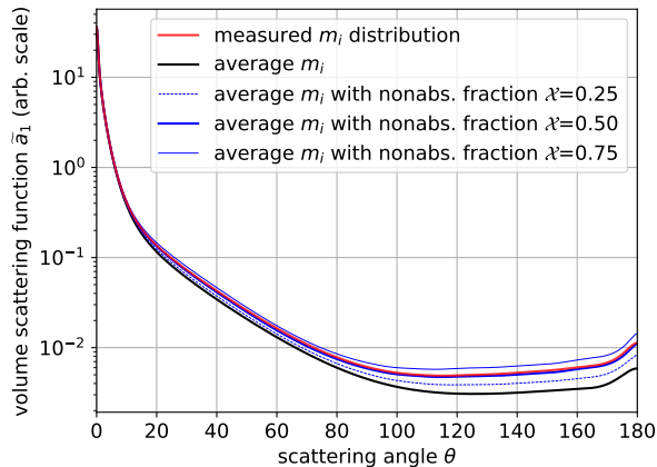
Figure 9. Volume scattering function of dust at \lambda = 355 nm (arbitrary scale) using either the m_i distribution (red) measured by Kandler et al. (2011), the average m_i of these measurements (black), or applying the non-absorbing fraction parameterization with different \mathcal{X} (blue).
