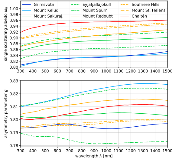
Figure 11. Modeled wavelength-dependent optical properties for ashes from different volcanoes. More details on the ash samples is given in Tab. Table 1 of Vogel et al. (2017). The colors indicate ash type: basalt in dark blue, basaltic andesite in light blue, andesite in green, dacite in orange, and rhyolite in red (see Fig. 7 of Vogel et al. (2017) for reference).
