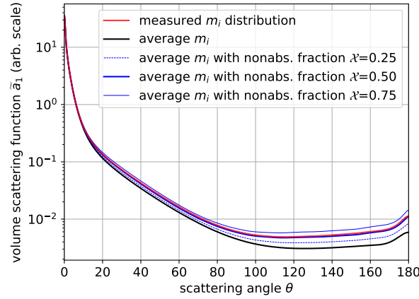
Figure 9. Volume scattering function of dust at \lambda=355 nm \lambda=355 nm (arbitrary scale) for different using either the m_i distributions distribution (see-textred) measured by Kandler et al. (2011), the average m_i of these measurements (black), or applying the non-absorbing fraction parameterization with different \mathcal{X} (blue).
