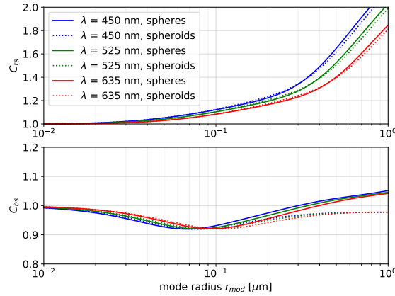
Figure 10. Modelled -Modeled correction factors C_{ts} for total scattering (upper plot) and C_{bs} for hemispheric backscattering (lower plot) of a Aurora 3000 nephelometer as function of particle size. For details see text.
