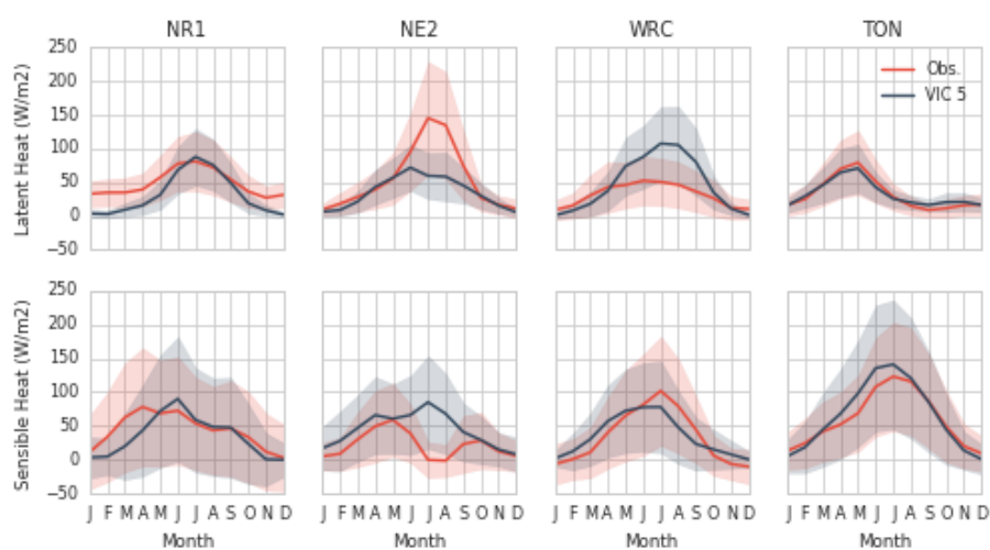
Figure 3. Example summary output from the VIC-5 science testing package comparing the annual cycle of latent heat (top) and sensible heat (bottom) for four sample locations for VIC-5 (blue) to FluxNet observations (red).
