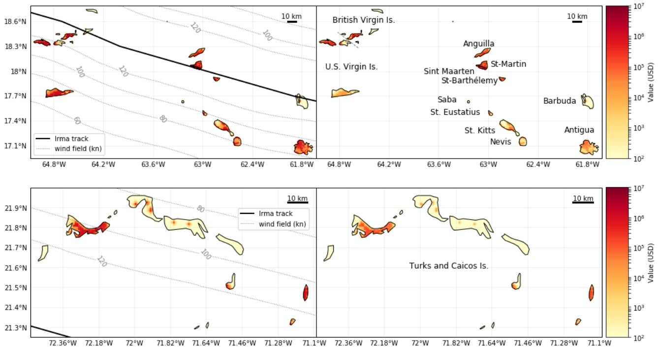
Figure 3: Left panels: rendered exposed value, contour lines of Irma maximum 1 min sustained winds (in knots) and Irma track. Right panels: economic damage generated by Irma.
