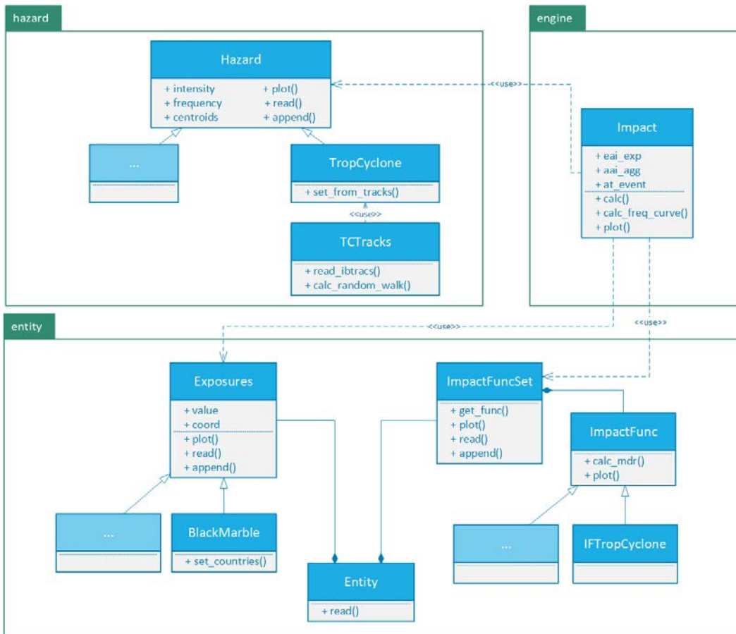
Figure 2: Simplified risk assessment architecture of CLIMADA. See Section 3 for more details on BlackMarble and TropCyclone. See for more information on CLIMADA’s components https://climada-python.readthedocs.io/en/latest/ .
