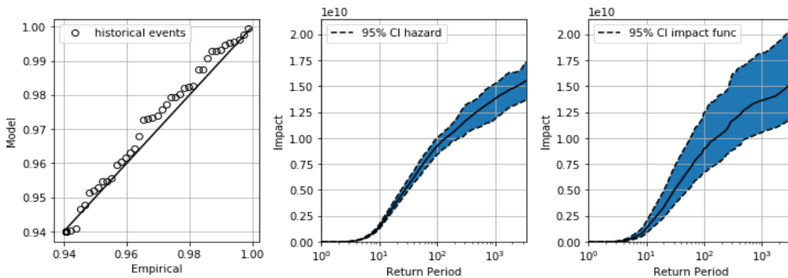
Figure 7: Quality metrics of the impact distribution. The left panel shows the probability-probability plot. The middle panel shows the mean value and the 95% confidence interval (CI) when sampling on the hurricane tracks and the right panel represents the 95% CI when sampling on impact functions with a maximal 10% shape modification, allowing to assess the uncertainty introduced by the models.
