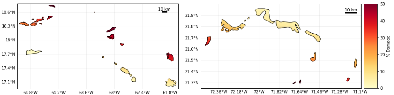
Figure 4: Economic damage as percentage of total local exposure (per pixel). Left panel: Lesser Antilles; right panel: Turks and Caicos Islands.
