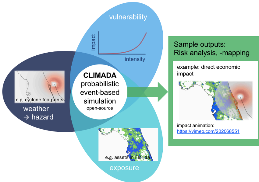
5 Figure 1: In essence, CLIMADA implements the concept of risk as in IPCC, 2014. CLIMADA combines hazard (e.g. a tropical cyclone wind footprint, leftmost inset), exposure (e.g. an asset distribution, centre bottom inset) and vulnerability (functional relationship between hazard intensity and impact, centre at the top) to calculate risk. Severity, measured e.g. as direct economic impact, is rendered by the red dots on the right panel. Please refer to the link provided for an animated version.
