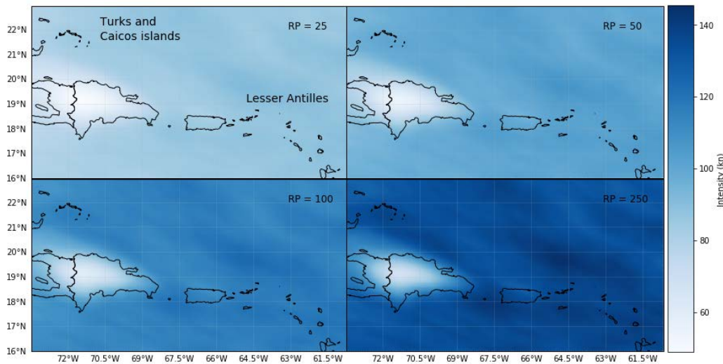
Figure 5: Wind fields in knots for return periods (RP) of 25, 50, 100 and 250 years in the study region.
