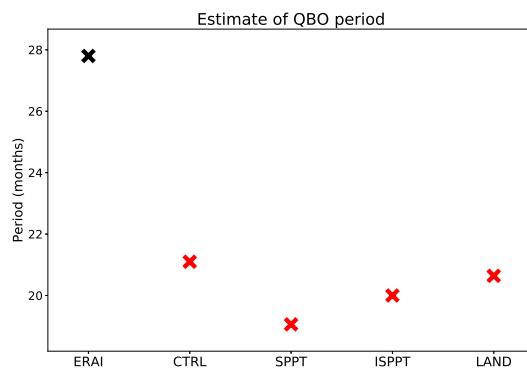
Figure 10. Estimate of the QBO period, as measured using equatorial zonal winds at 50hPa. The reanalysis product ERA-Interim is shown for comparison.
