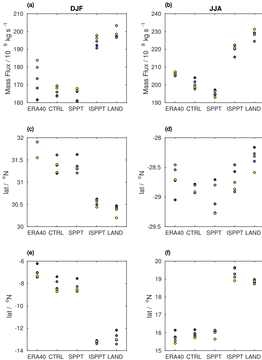
Figure 9. Impact of stochastic parametrizations on the Hadley circulation. The magnitude of the overturning circulation indicated by the maximum of the streamfunction of the dominant cell in (a) DJF and (b) JJA for each scheme. The latitude of the downwelling branch of the dominant (winter hemisphere) cell in (c) DJF and (d) JJA. The latitude of the upwelling branch of the dominant (winter hemisphere) cell in (e) DJF and (f) JJA. The data diagnostic is shown for each of the five AMIP simulations in turn, the darker colours indicate earlier years, ranging from dark blue (1960–1980) to yellow (1980–2000).
