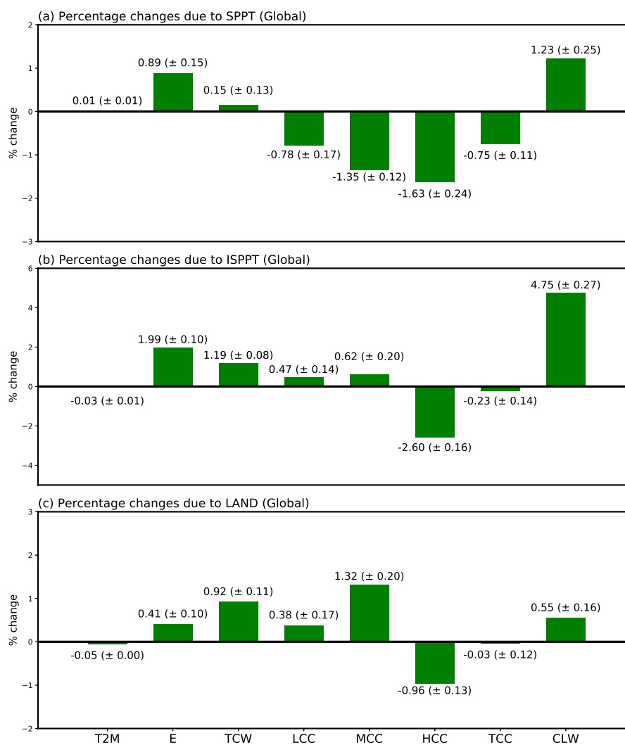
Figure 1. Average percentage change, relative to CTRL, in global mean of (a) SPPT simulations, (b) ISPPT and (c) LAND. Variables shown are, in order, two-meter temperature (T2M), evaporation (E), total column water (TCW), low cloud cover (LCC), mid-level cloud cover (MCC), high-level cloud cover (HCC), total cloud cover (TCC) and cloud liquid water (CLW). Uncertainty estimates are twice the standard deviation of the five individual differences. Note: due to conservation of water, the change in precipitation (not shown) is almost exactly equal to the change in evaporation.
