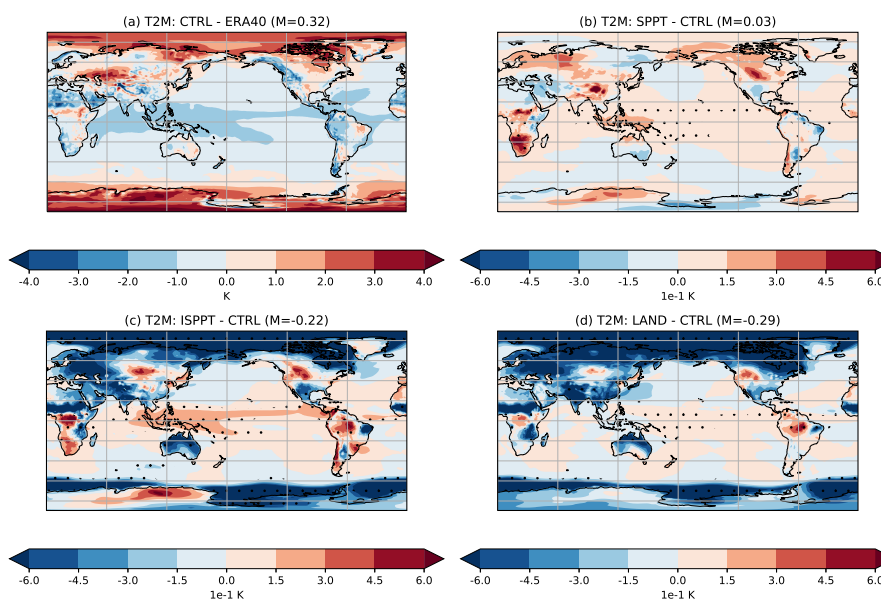
Figure 6. Mean differences in two-meter temperature between (a) CTRL and ERA40, (b) SPPT and CTRL, (c) ISPPT and CTRL and (d) LAND and CTRL. Stippling indicates regions where the difference is statistically significant to the 95% confidence interval, as measured by a two-tailed T-test. Note the difference in scales between (a) and (b)-(c)-(d).
