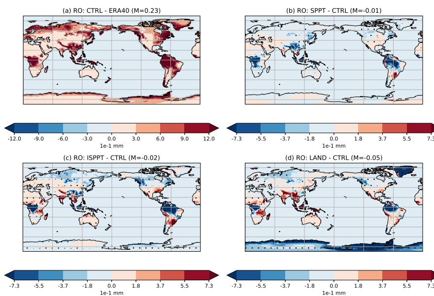
Figure 5. Mean differences in runoff between (a) CTRL and ERA40, (b) SPPT and CTRL, (c) ISPT and CTRL and (d) LAND and CTRL. Stippling indicates regions where the difference is statistically significant to the 95% confidence interval, as measured by a two-tailed T-test. Note the difference in scales between (a) and (b)-(c)-(d).
