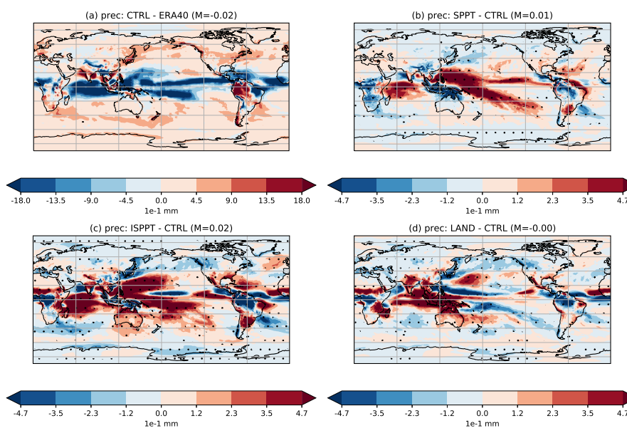
Figure 4. Mean differences in precipitation between (a) CTRL and ERA40, (b) SPPT and CTRL, (c) ISPPT and CTRL and (d) LAND and CTRL. Stippling indicates regions where the difference is statistically significant to the 95% confidence interval, as measured by a two-tailed T-test. Note the difference in scales between (a) and (b)-(c)-(d).
