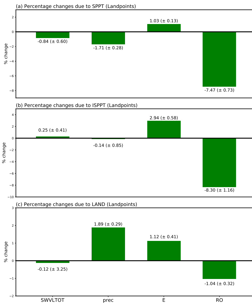
Figure 2. Average percentage change, relative to CTRL, in global mean of (a) SPPT simulations, (b) ISPPT and (c) LAND. All data was restricted to land-points only. For LAND, Antarctica was also excluded. Variables shown are, in order, total soil water content (SWVLTOT), precipitation (prec), evaporation (E) and runoff (RO). Uncertainty estimates are twice the standard deviation of the five individual differences.
