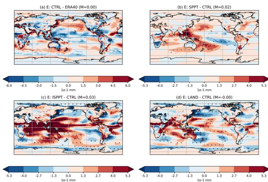
Figure 3. Mean differences in evaporation between (a) CTRL and ERA40, (b) SPPT and CTRL, (c) ISPPT and CTRL and (d) LAND and CTRL. Stippling indicates regions where the difference is statistically significant to the 95% confidence interval, as measured by a two-tailed T-test. Note the difference in scales between (a) and (b)-(c)-(d).
