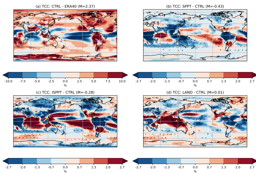
Figure 7. Mean differences in total cloud cover between (a) CTRL and ERA40, (b) SPPT and CTRL, (c) ISPPT and CTRL and (d) LAND and CTRL. Stippling indicates regions where the difference is statistically significant to the 95% confidence interval, as measured by a two-tailed T-test. Note the difference in scales between (a) and (b)-(c)-(d). The units of % indicate the proportion of the column occupied by clouds.
