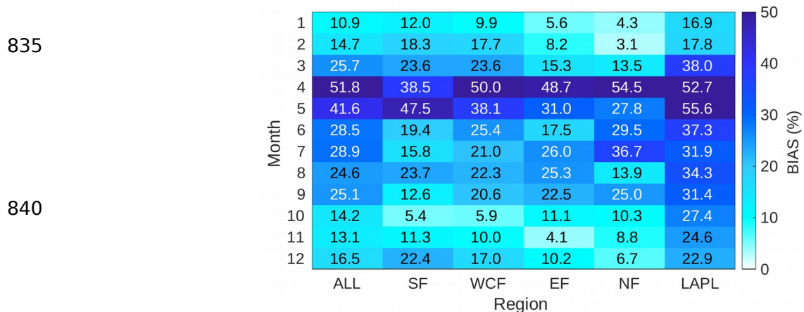
840 845 Figure 7: The monthly mean biases of simulated precipitation averaged over (a) Southern Finland (SF), (b) Western and Central Finland (WCF), (c) Eastern Finland (EF), (d) Northern Finland (NF), (e) Lapland (LAPL), and (f) the whole Finland (ALL) in 2002–2014 with a reference to E-OBS.
