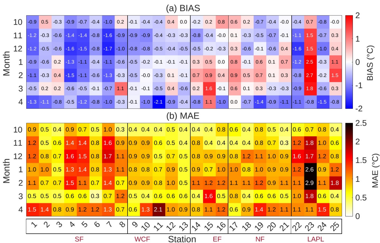
Figure 9: (a) The mean monthly biases and MAE values of simulated road surface temperature between October and April in 2002–2014. The station indices on the x-axis refer to Table 1. SF refers to Southern Finland, WCF to Western and Central Finland, EF to Eastern Finland, NF to Northern Finland, and LAPL to Lapland.
