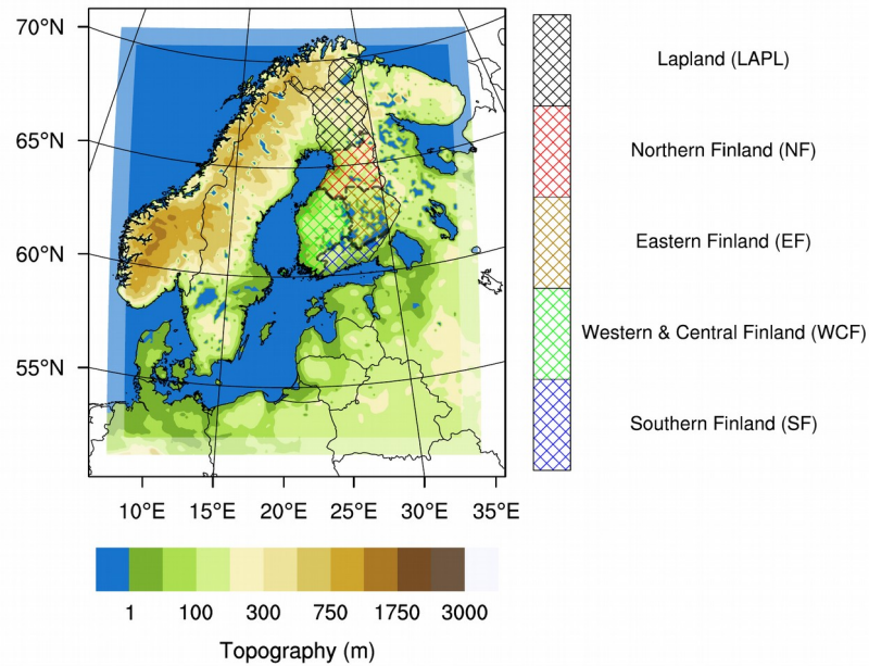
Figure 1: The HCLIM38-ALARO model domain and topography at 12.5 km x 12.5 km grid resolution. Colored overlays depict the regions that are evaluated in more detail. The transparent areas depict the model's 8-point wide relaxation zone.
