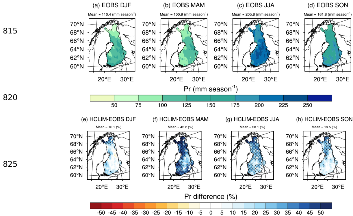
825 830 Figure 6: (a–d) The reference values of precipitation ( Pr ) from E-OBS data and (e–h) the biases of HCLIM38-ALARO modeled Pr with a reference to E-OBS. The seasonal averages were calculated for the time period of January 2002–December 2014. Stippled areas represent statistically significant differences with p values < 0.05 .
