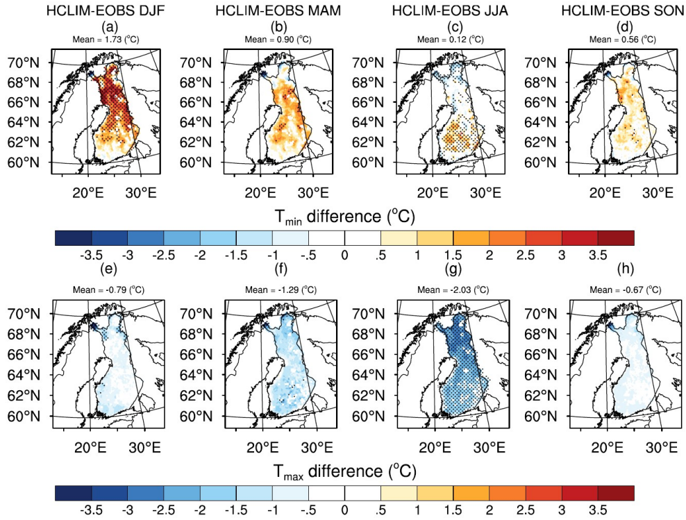
Figure 5: The biases in the simulated seasonal means of (a–d) minimum near-surface air temperature ( T_{min} ) and (e–h) maximum near-surface air temperature ( T_{max} ) with a reference to E-OBS. The seasonal mean biases were calculated over Finland for the time period of January 2002–December 2014. Stippled areas represent statistically significant differences with p values < 0.05.
