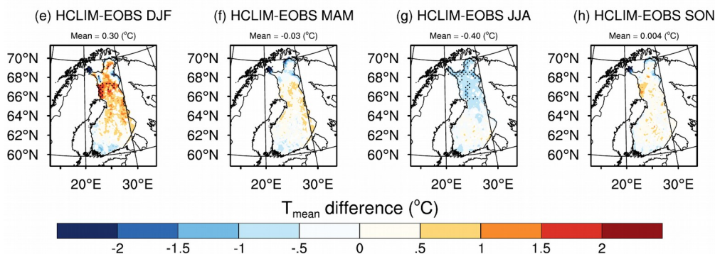
Figure 3: (a–d) The reference values of mean near-surface air temperatures ( T_{mean} ) from E-OBS data and (e–h) the biases of HCLIM38-ALARO modeled T_{mean} with a reference to E-OBS. The seasonal means were calculated over the whole model domain for the time period of January 2002–December 2014. Stippled areas represent statistically significant differences with p values < 0.05 .
