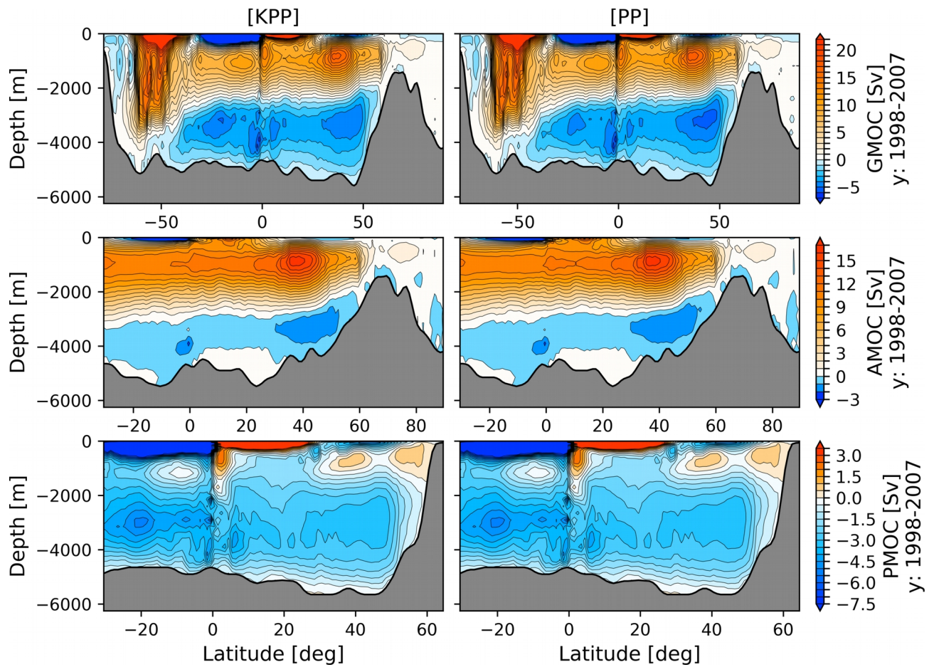
Suppl. 2: Global (GMOC, upper row), Atlantic (AMOC, middle row) and Indo-Pacific (PMOC, lower row) Meridional Overturning Circulation averaged for the time period 1998-2007 for the simulations with KPP (left column) and PP (right column) vertical mixing.
