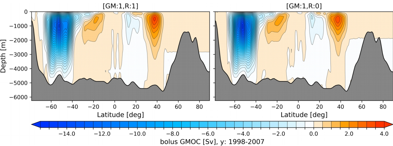
Suppl. 1: Global Meridional Overturning Circulation (GMOC) calculated from Gent McWilliams vertical bolus velocity, averaged for the time period 1998-2007, for the reference simulation (left) and the simulation in which the Redi diffusivity is set to zero (right).
