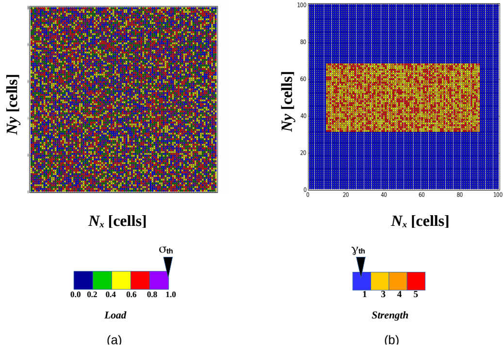
Figure 3. (a) Spatial distribution of the random initial loads \sigma(i, j) . R_{A_{sp}} represents a rectangular fault plane of N_x = N_y = 100 cells. The color bar indicates the load and the threshold load of \sigma_{th} = 1 . (b) Spatial distribution of the strength \gamma(i, j) . Two main regions can be distinguished in this figure: 1) the asperity region defined as the inner rectangle, and 2) a background area or fault plane. While the asperity contains strength values in the range of 3 to 5, the rest of the fault plane has a strength value of 1.
