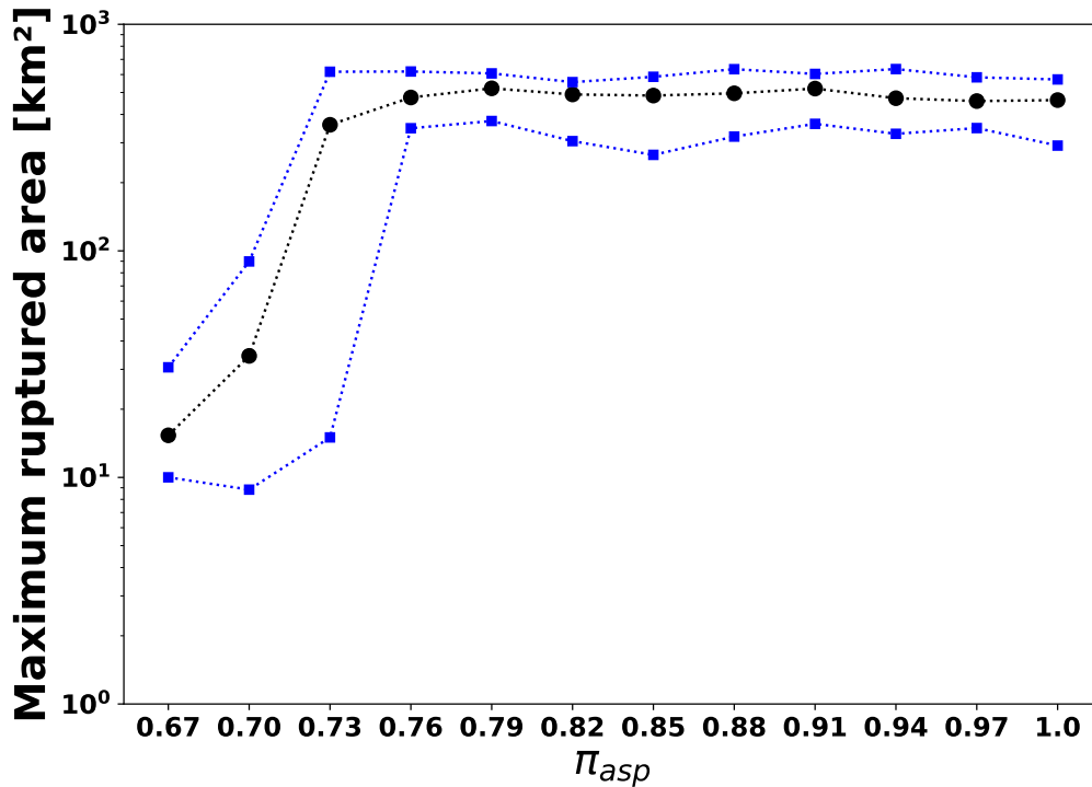
Figure 9. Mean of the maximum rupture area [km 2 ], A_{syn} for different values of \pi_{asp} depicted as black circles. The minimum and maximum limits of the rupture area are represented by blue squares.
