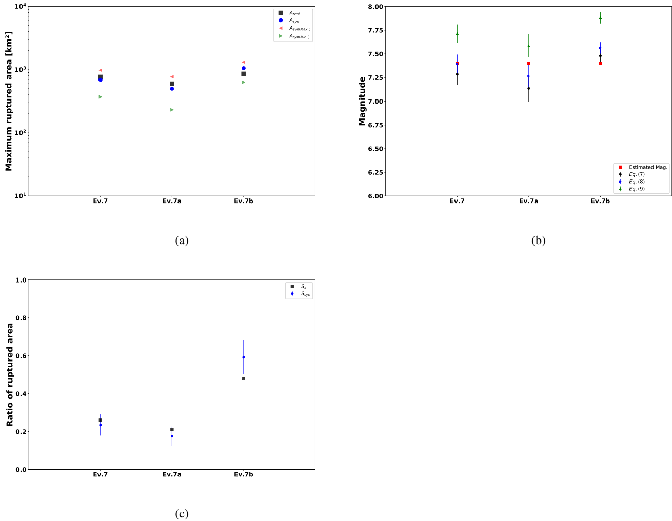
Figure 19. A comparison between the data from table 5 and the results by TREMOLO for the events 7, 7a and 7b. (a) Maximum ruptured area, A_{syn} ; (b) mean maximum magnitude, M_{syn} ; (c) ratio of maximum event size S_{syn} .
