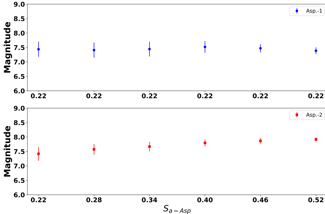
Figure 13. Statistical results of S_a - A_{sp} for a configuration similar to figure 7. The markers indicate mean and standard deviation for 50 realizations. Red markers correspond to the results of the right and variable asperity and blue markers to the results of the right and stable asperity.
