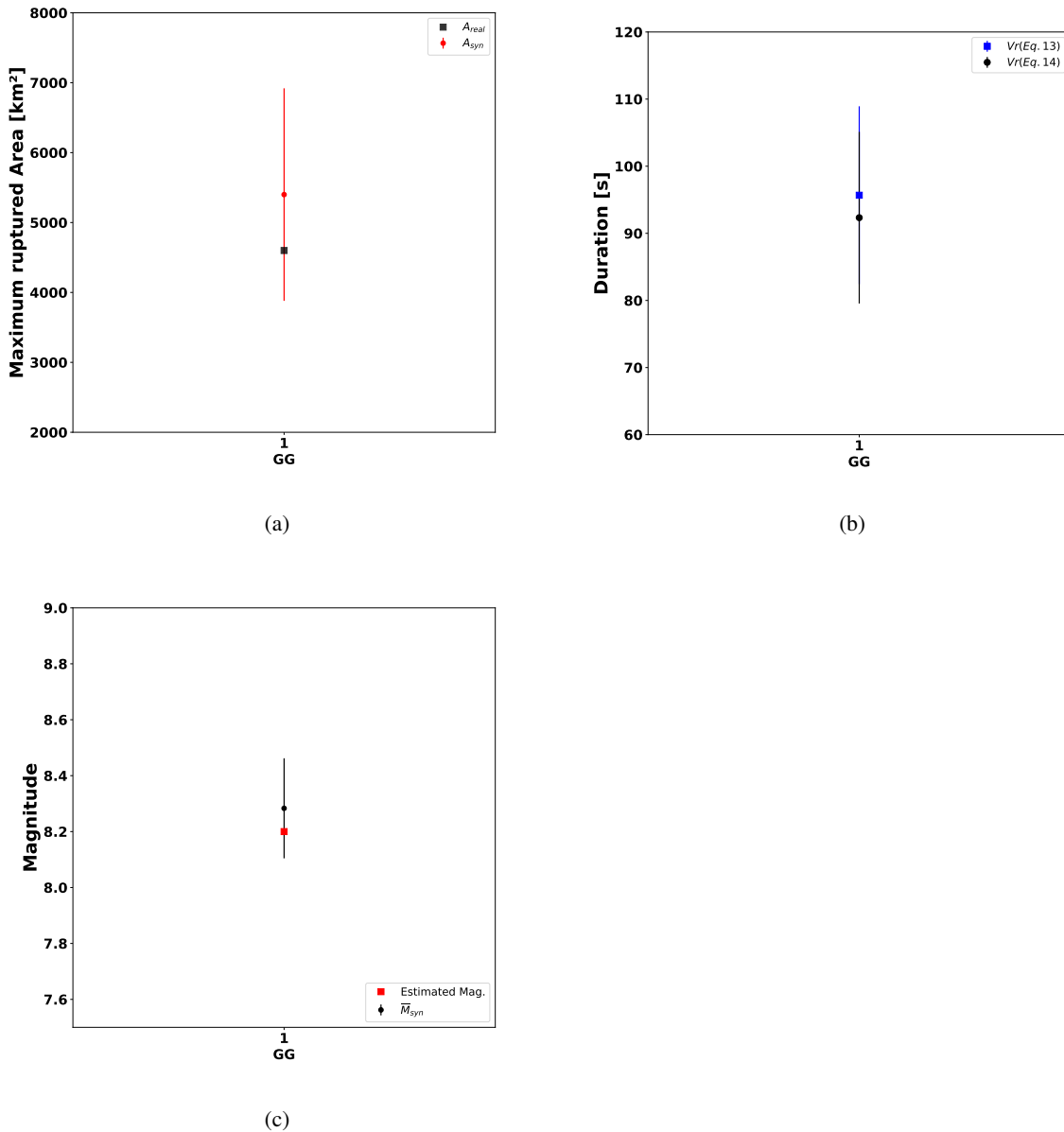
Figure 20. Estimation of the characteristics of a future earthquake in the Guerrero seismic gap. (a) estimated rupture area, (b) rupture duration, (c) average of the mean magnitude considering three scale relations Eqs. 7, 8, and 9.
