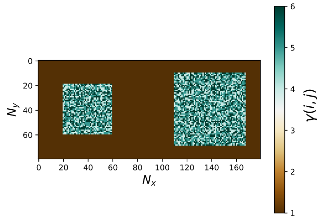
Figure 7. An example configuration of different asperity sizes, S_{a-ASP} . The color bar indicates the strength \gamma(i, j) values used during the test.
