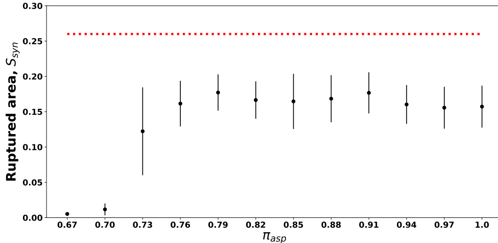
Figure 11. Mean and standard deviation of the ratio S_{\text{syn}} = A_{\text{syn}}/A_{\text{eff}} over 50 realizations for different values of \pi_{\text{asp}} . The red line indicates the asperity ratio S_a computed for event 7 (Table 5).
