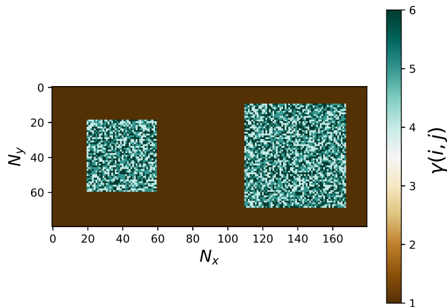
Figure 7. An example configuration of different asperity sizes, S_{\text{a-Asp}} . The color bar indicates the strength \gamma(i, j) values used during the test.
