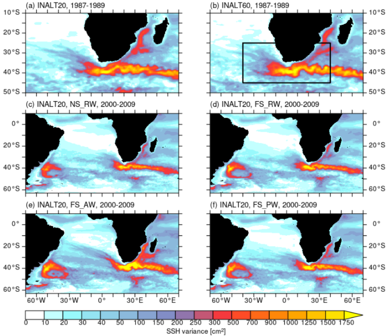
Figure 4. SSH variance [in \text{cm}^2 ] for the period 1987 to 1989 from the spin-up experiments in (a) INALT20 and (b) INALT60 based on 5-day averages; The black box in (b) marks the region of the secondary 1/60^\circ nest in INALT60. (c to f) give the SSH variance [in \text{cm}^2 ] for the period 2000-2009 based on 5-day averages from the different sensitivity experiments in INALT20: (c) no slip, relative winds, (d) free slip, relative winds, (e) free slip, absolute winds, (f) free slip, partial winds.
