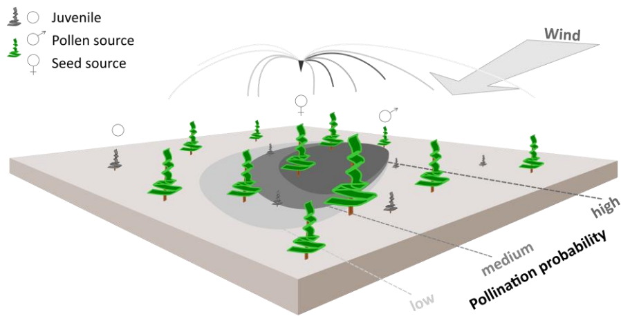
685 Figure 1. Schematic representation of wind pollination as newly implemented in the LAVESI-WIND model. Based on actual winds, a distance-dependent pollination probability of ovules is estimated for each adult tree (potential pollen source) and for each seed source in the simulated area. The shaded areas on the ground represent the pollination probability for the labelled seed source for winds from the upper-right corner. These are generally higher for adult trees in upwind direction of the central seed source.
