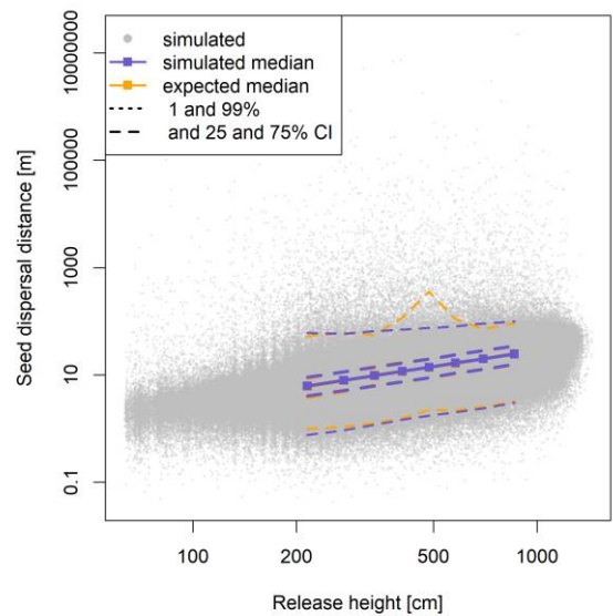
690 Figure 2. Dispersal distances of seeds are wind dependent and positively correlated with the height of the releasing tree. The simulated and hypothetically calculated dispersals were compared across evenly distributed height classes; the results are similar for north and south winds, and here the results with north winds are presented.
