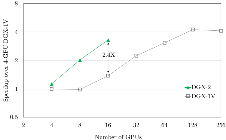
Figure 7. Computational performance of the spectral transform dwarf at 18km resolution ( N_T = 639 ) on up to 16 GPUs on one DGX-2 and up to 32 DGX-1 servers connected with Infiniband. The DGX-1V uses MPI for \geq 8 GPUs (due to lack of AlltoAll links), all others use CUDA IPC. DGX-2 results use pre-production hardware. The points were connected with lines for the purpose of improving readability.
