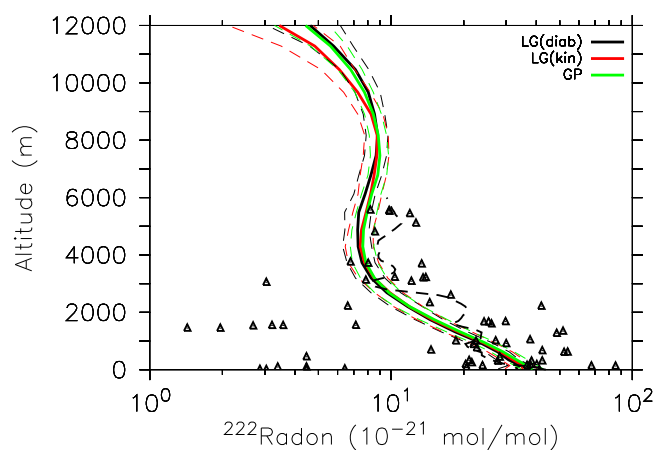
Figure 5. Vertical profiles of ^{222}\text{Rn} mixing ratio [ 10^{-21} mol/mol] during the NARE campaign. Dashed lines represent the one \sigma standard deviation of the simulations. The thick dashed line is a spline interpolation of the scattered data on the grid.
