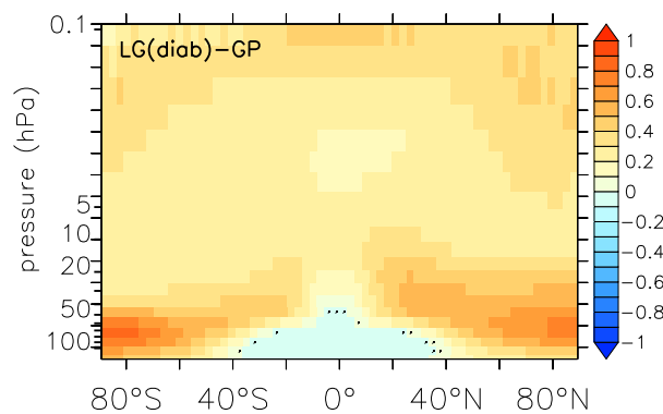
Figure 9. Zonal mean difference of AoA (LG(diab)-GP) from SF 6 -AoAc tracer (with constant source of SF 6 at the surface). NOT stippled area is statistically significant to the 99% level
