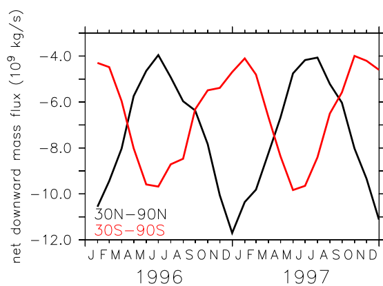
Figure 15. Monthly net mass fluxes (downward) from LG(diab) simulations through the 380 K isentropes for the northern and southern extra-tropics.
