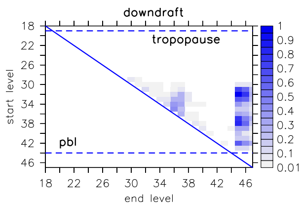
Figure 17. Movement characteristic of parcels, which are transported in the downdraft in 1997. The vertical axis describes the start model level of a parcel. The horizontal axis describes the respective final downdraft levels.
