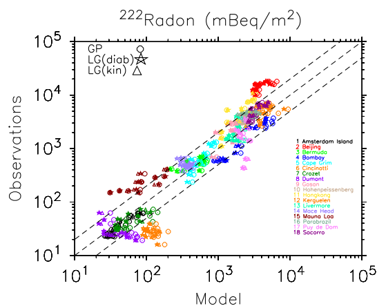
Figure 4. Monthly mean ^{222}\text{Rn} [ \text{mBeq/m}^2 ] surface concentrations: GP and LG model results against observations at different sites from Zhang et al. (2008). The thick dashed lines include a range within a factor of two of the observations.
