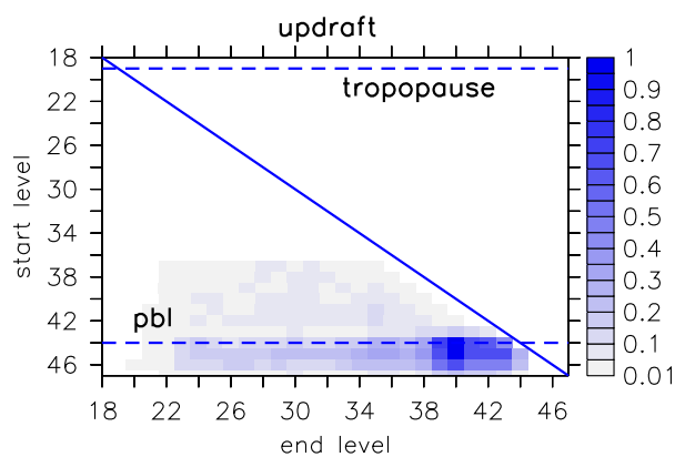
Figure 16. Movement characteristic of parcels, which are transported in the updraft in 1997. The vertical axis describes the start model level of a parcel. The horizontal axis describes the respective final updraft levels.
