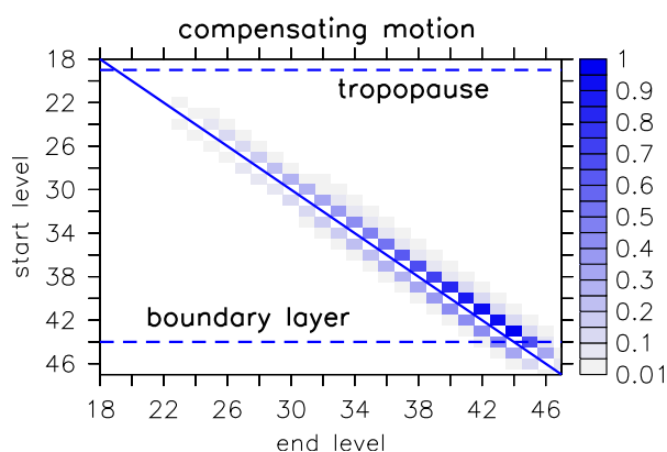
Figure 18. Movement characteristic of parcels, which represents the compensating movement in the environment (subsidence) in 1997. The vertical axis describes the start model level of a parcel. The horizontal axis describes the respective final subsidence levels. Note, that also a compensating upward parcel movement exist (shown below the blue diagonal line). For details see text.
