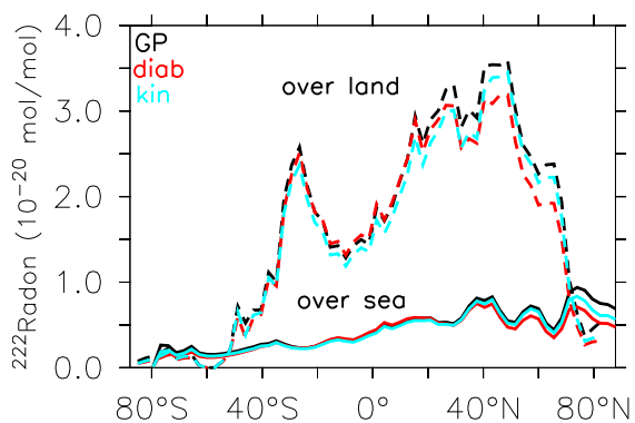
Figure 3. Zonal mean ^{222}\text{Rn} concentration between 800 and 1013 hPa (weighted by the level thickness) over land (dashed) and over sea (solid) for GP (black line), LG(diab) (red line) and LG(kin) (light blue line).
