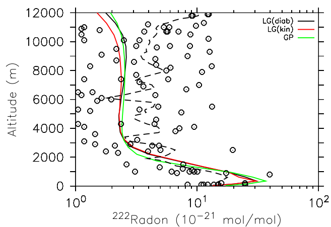
Figure 6. Vertical profiles of ^{222}\text{Rn} mixing ratio [ 10^{-21}\text{mol/mol} ] during the MOFFET campaign. The thick dashed line is a spline interpolation of the scattered data on the grid.
