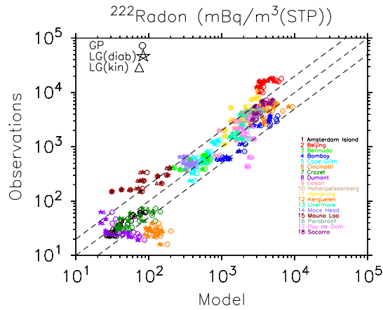
Figure 4. Monthly mean ^{222}\text{Rn} \text{mBq m}^{-3}(\text{STP}) surface concentrations: GP and LG model results against observations at different sites from Zhang et al. (2008). The thick dashed lines include a range within a factor of two of the observations.
