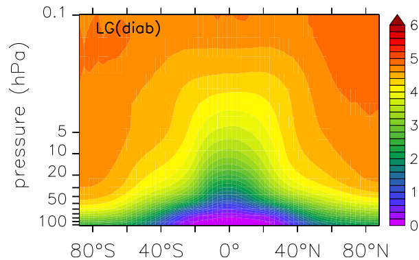
Figure 8. Zonal mean AoA (in years) from SF 6 -AoA of the LG(diab) simulation.
