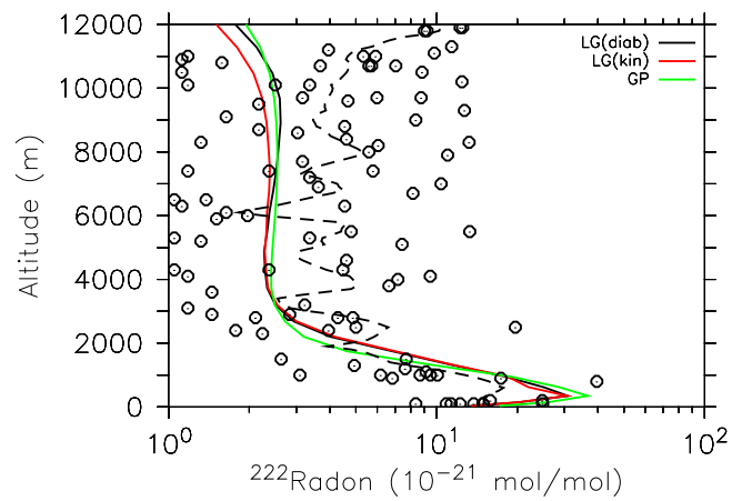
Figure 6. Vertical profiles of ^{222}\text{Rn} mixing ratio [ 10^{-21} mol/mol] during the MOFFET campaign. The thick dashed line is a spline interpolation of the scattered measurement data (circles) on the grid.
