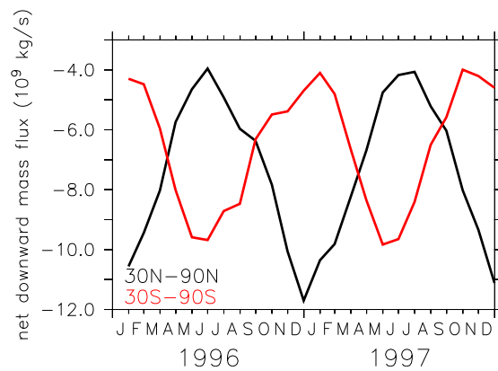
Figure 15. Monthly net mass fluxes from LG(diab) simulation through the 380 K isentrope for the northern and southern extra-tropics.
