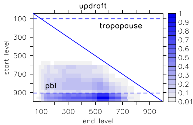
Figure 16. Movement characteristic of parcels, which are transported in the updraft in 1997. The vertical axis describes the start level of a parcel, the horizontal axis describes the respective final updraft (end) level. Displayed are the respective number of parcels transported in the updraft, normalised with the maximum number.
