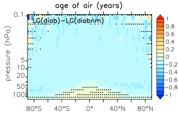
Figure 12. Zonal mean difference between LG(diab) with standard mixing of SF 6 -AoA tracer and LG(diab) with no-mixing (nm) between adjacent parcels. NOT stippled area is statistically significant to the 99% level.
