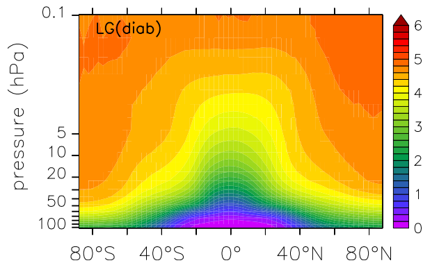
Figure 8. Zonal mean AoA (in years) from SF 6 -AoA of the LG(diab) simulation.
