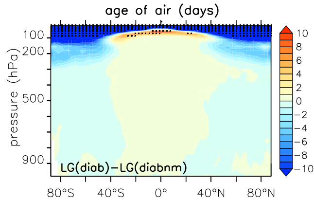
Figure 13. Zonal mean difference between LG(diab) and LG(diab-nm) with no inter-parcel mixing. STIPPLED area is statistically significant to the 99% level.
