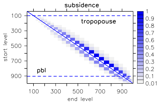
Figure 18. Similar as Fig. 16 but for parcels representing the compensating movement in the environment (subsidence) in 1997. Note, that also a compensating upward parcel movement exist (shown below the blue diagonal line). For details see text.
