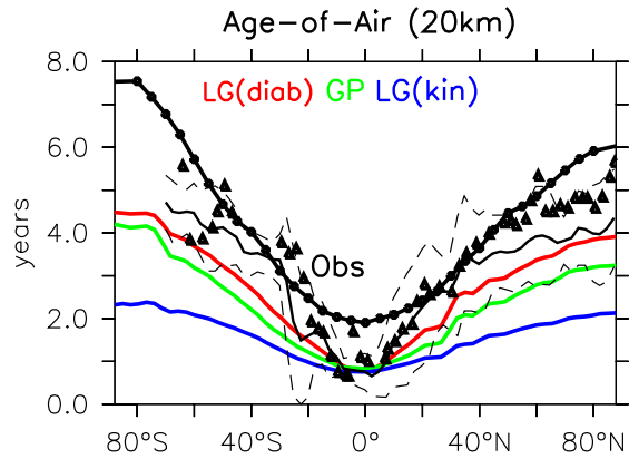
Figure 7. Zonal mean AoA at 20 km height ( \sim 50 hPa) from SF 6 -AoA tracer (red: LG(diab), green: GP, blue: LG(kin)), a mean over the years 2000-2010. Thick black line with circles: MIPAS data, a mean over the years 2003, 2007, 2008, 2009, 2010, 2011. Triangles: AoA from SF 6 at 20 km, from Waugh and Hall (2002). Thin black dashed lines: minimum and maximum AoA from CO 2 at 20 km from Andrews et al. (2001).
