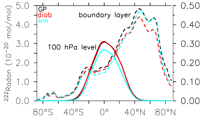
Figure 2. Zonal mean ^{222}\text{Rn} mixing ratio in the boundary layer (averaged over the lowest three model layers, dashed, left vertical axis) and at 100 hPa (solid, right vertical axis). GP denotes the grid point simulation with EMAC (black line), LG(diab) the simulation with EMAC-ATTILA using the diabatic vertical velocity (red line), and LG(kin) the EMAC-ATTILA simulation with kinematic vertical velocity (light blue line).
