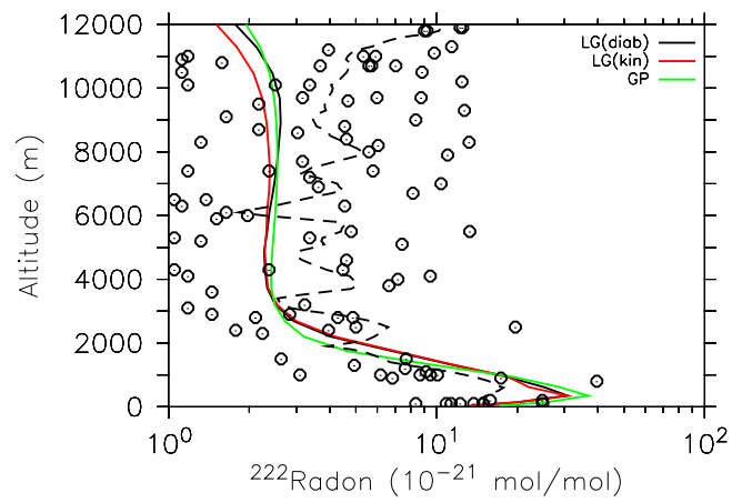
Figure 6. Vertical profiles of ^{222}\text{Rn} mixing ratio [ 10^{-21} mol/mol] during the MOFFET campaign. The thick dashed line is a spline interpolation of the scattered measurement data (circles) on the grid.
