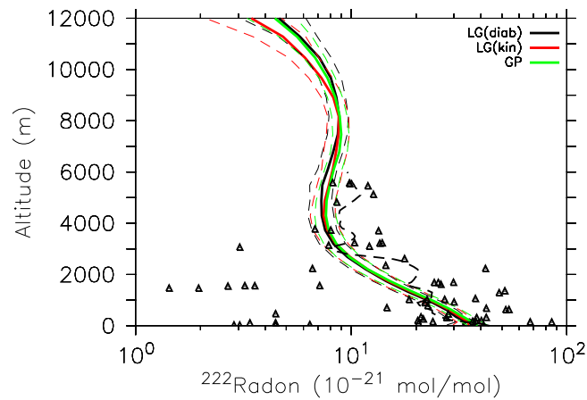
Figure 5. Vertical profiles of ^{222}\text{Rn} mixing ratio [ 10^{-21} mol/mol] during the NARE campaign. The thick dashed line (limited to a height of 6000 m) is a spline interpolation of the scattered measurement data (triangles) on the grid. Thin dashed lines represent the one \sigma standard deviation of the respective simulations.
