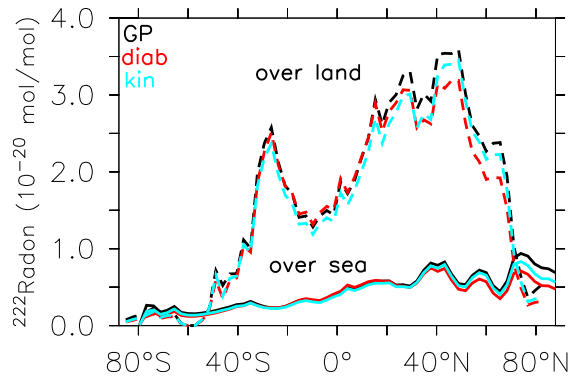
Figure 3. Zonal mean ^{222}\text{Rn} mixing ratio between 800 and 1013 hPa (weighted by the level thickness) over land (dashed) and over sea (solid) for GP (black line), LG(diab) (red line) and LG(kin) (light blue line).
