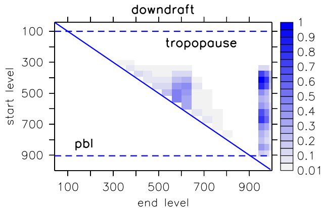
Figure 17. Similar as Fig. 16 but for parcels, which are transported in the downdraft in 1997.
