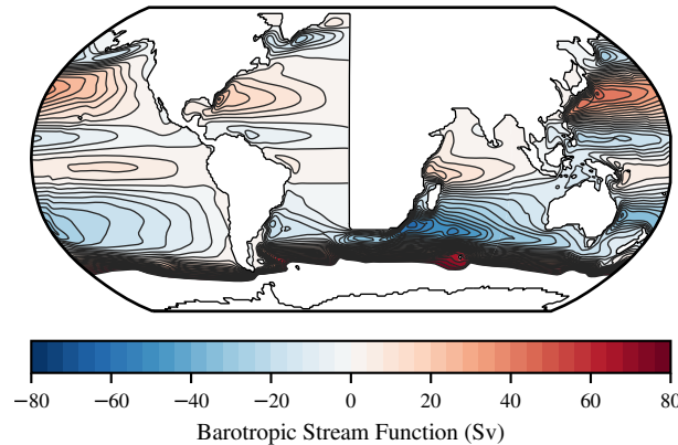
Figure 4. Long-term average barotropic stream function (BSF) of a 1^\circ \times 1^\circ horizontal resolution setup as described in Sect. 4.1. 1\text{ Sv} = 10^6 \text{ m}^3\text{s}^{-1} . Contours are drawn in steps of 4\text{ Sv} .
