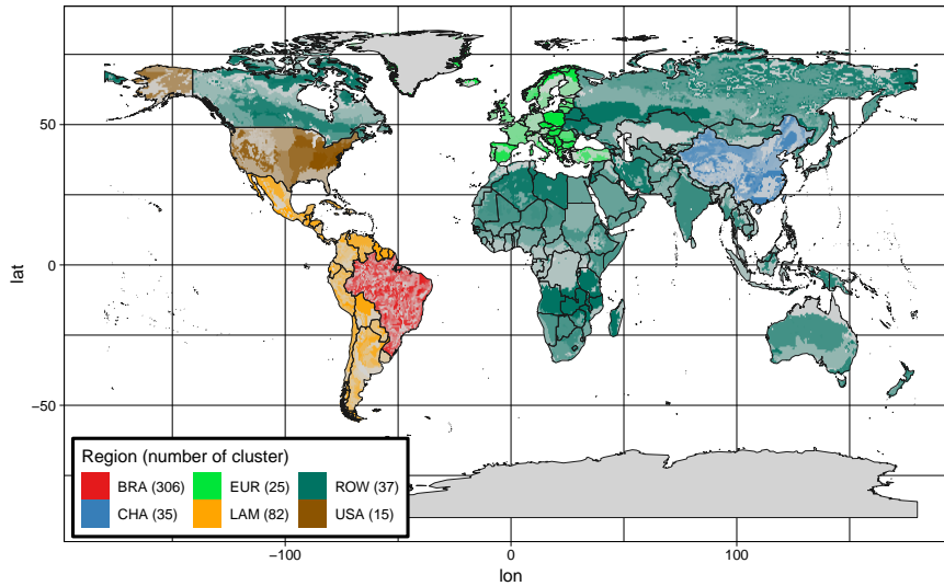
Figure 4. Study setup tailored to assessments with a focus on Brazil, with 6 world regions and 500 clusters : Brazil (BRA) in increased spatial resolution, its major trade partners Latin America (LAM), United States (USA), China (CHA) and Europe (EUR) in default resolution and rest of the world (ROW) combined to one region with reduced resolution.
