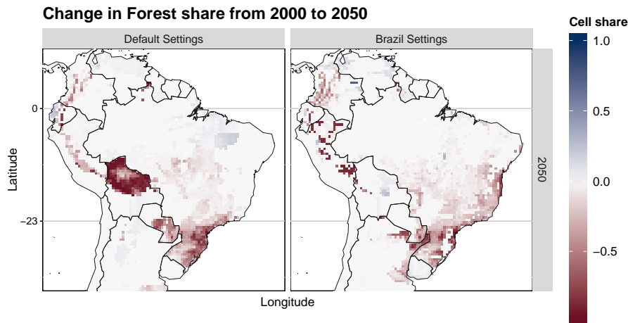
Figure 6. Comparison of changes in forest share from 2000 to 2050 in Brazil between default setup and Brazil setup.
