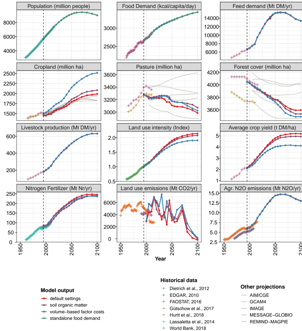
Figure 2. Evaluation plots for MAGPIE 4 inputs and outputs for SSP1-5 reference scenarios at global level the default settings, a run with soil organic matter explicitly modeled, a run with an alternative factor requirement setup with costs proportional to the production volume and a standalone run of the food demand module. Sources of historical data: (Canadell et al., 2007; Dietrich et al., 2012; EDGAR, 2010; FAOSTAT, 2016; Harris et al., 2012; Hurt et al., 2018; Gütschow et al., 2017; World Bank, 2018) (Dietrich et al., 2012; EDGAR, 2010; FAOSTAT, 2016; Gütschow et al., 2017; Hurt et al., 2018; Lassaletta et al., 2014; World Bank, 2018) . Sources of other projections for SSP1-5 SSP2 reference scenarios scenario: (IAMC, 2016).
