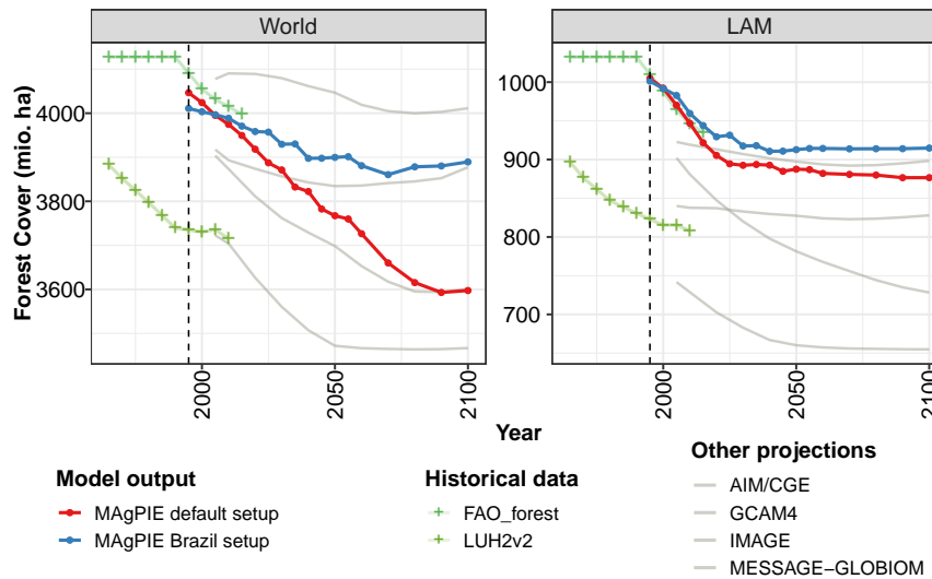
Figure 5. Comparison of global and Latin American forest cover with historical data sets and projections of other models.
