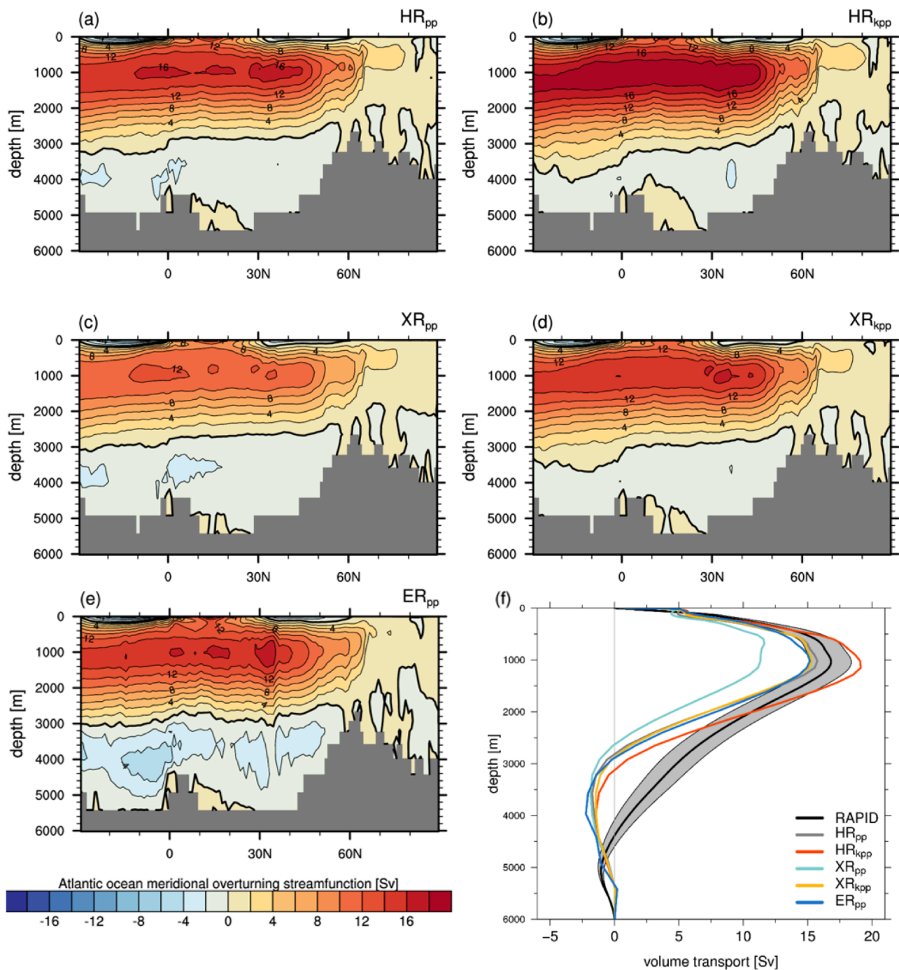
Figure 12. Eulerian stream function ( \text{Sv} := 10^6 \text{ m}^3 \text{ s}^{-1} ) of the Atlantic Meridional Overturning Circulation (AMOC) for (a) HR pp , (b) HR kpp , (c) XR pp , (d) XR kpp , and (e) ER pp . The zero contour is drawn as a thicker line. In (f) annual mean profiles of the AMOC at 26.5°N are shown as observed from Apr 2004 to Feb 2017 by the RAPID-MOCHA-WBTS array ( \pm one standard deviation marked by grey shading) (Smeed et al., 2017) and simulated by MPI-ESM1.2.
