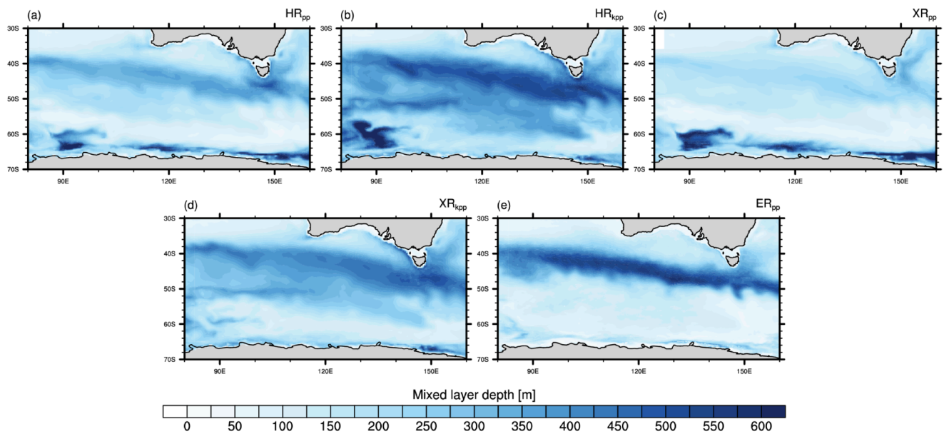
Figure A9. Time-averaged mixed layer depths ( \sigma_t = 0.03 \text{ kg m}^{-3} ) across the Subantarctic Frontal zone in September simulated by (a) HR pp , (b) HR kpp , (c) XR pp , (d) XR kpp , and (e) ER pp .
