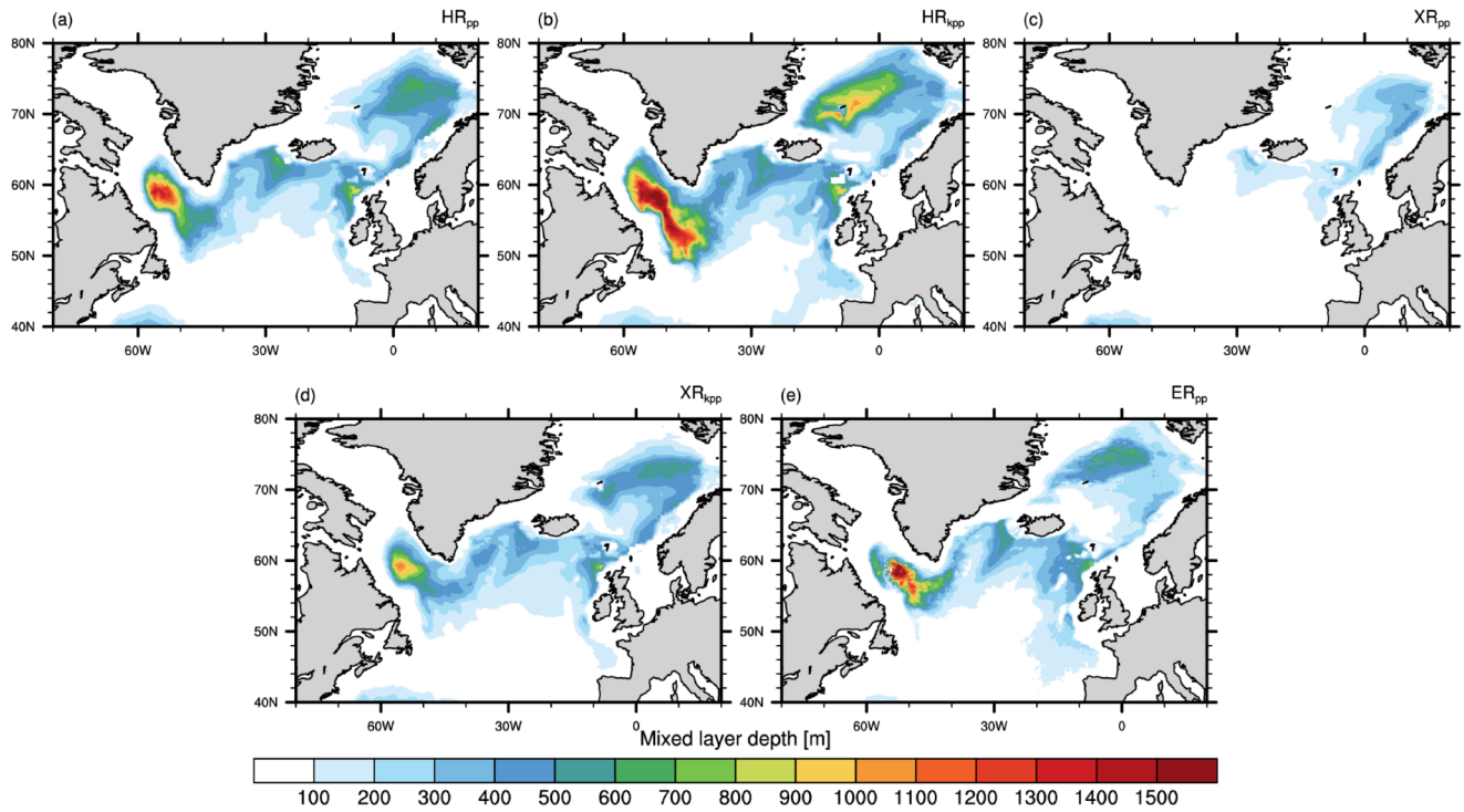
Figure 10. Time-averaged mixed layer depth ( \sigma_t = 0.01 \text{ kg m}^{-3} ) in March in the North Atlantic and the Nordic Seas for (a) HR_{pp} , (b) HR_{kpp} , (c) XR_{pp} , (d) XR_{kpp} , and (e) ER_{pp} .
