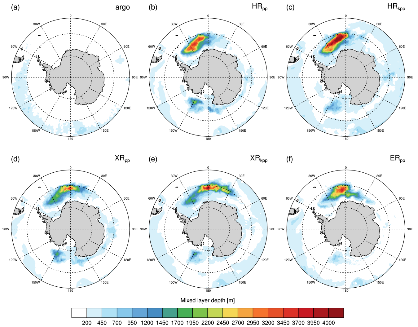
Figure 11. Time-averaged mixed layer depth ( \sigma_t = 0.03 \text{ kg m}^{-3} ) in September in the Southern Ocean [.. 46 ] from (a) 1^\circ \times 1^\circ gridded Argo float data (Holte et al., 2017) and from (b) HR pp , ([.. 47 ] (c) HR kpp , ([.. 48 ] (d) XR pp , ([.. 49 ] (e) XR kpp , and ([.. 50 ] (f) ER pp .
