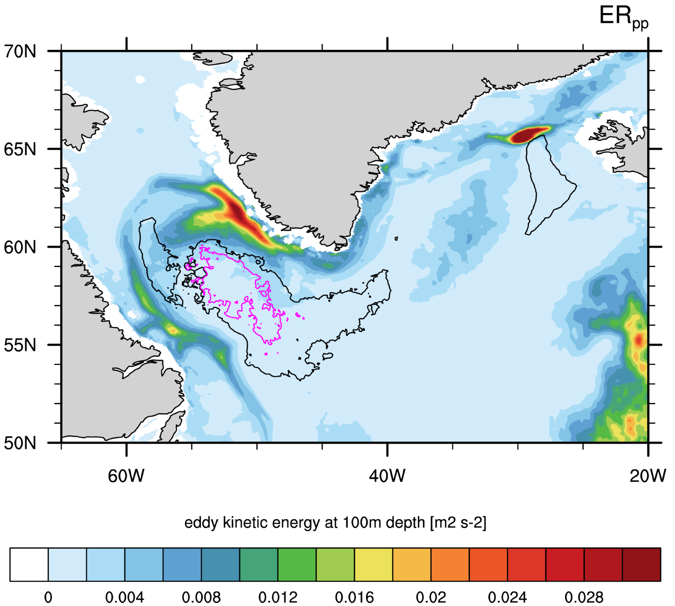
Figure A9. Time-averaged [.51] eddy kinetic energy ( [.52] eke = 1/2(\overline{u'^2 + v'^2}) in m^2 s^{-2} ) [.53] in [.54] March simulated by [.55] ER pp . In addition, the mean mixed layer depths in March are shown as contour lines ( [.56] black: 500 m and [.57] magenta: 1000 m) [.58] .
