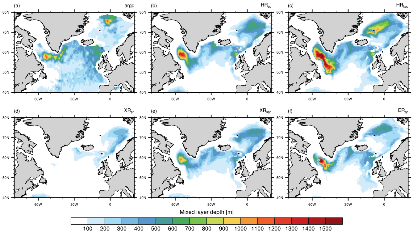
Figure 10. Time-averaged mixed layer depth ( \sigma_t = 0.01 \text{ kg m}^{-3} ) in March in the North Atlantic and the Nordic Seas [.. 41 ] from (a) 1^\circ \times 1^\circ gridded Argo float data (Holte et al., 2017) and from (b) HR pp , ([.. 42 ]c) HR kpp , ([.. 43 ]d) XR pp , ([.. 44 ]e) XR kpp , and ([.. 45 ]f) ER pp .
