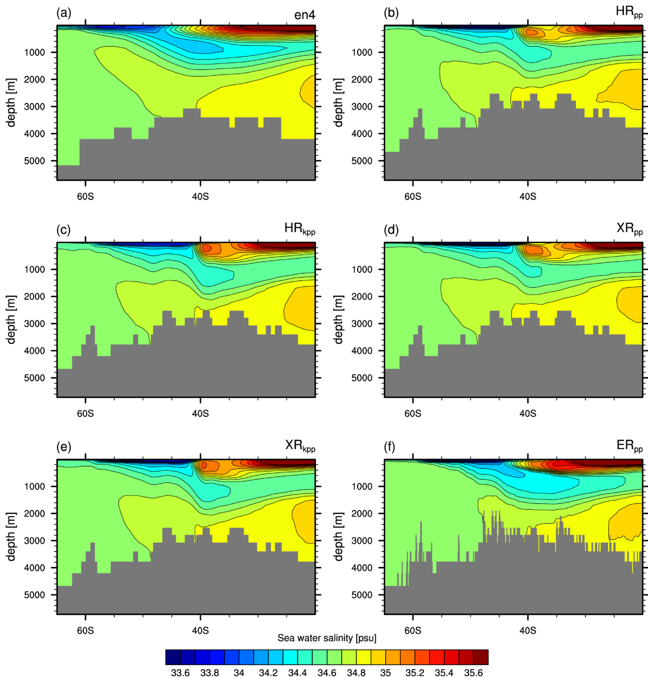
Figure A8. Time-averaged salinity section along 15^{\circ}\text{W} (from 65^{\circ}\text{S} to 20^{\circ}\text{S} ) in the Southern Ocean of (a) EN4 (1945-1955), (b) HR pp , (c) HR kpp , (d) XR pp , (e) XR kpp , and (f) ER pp .
