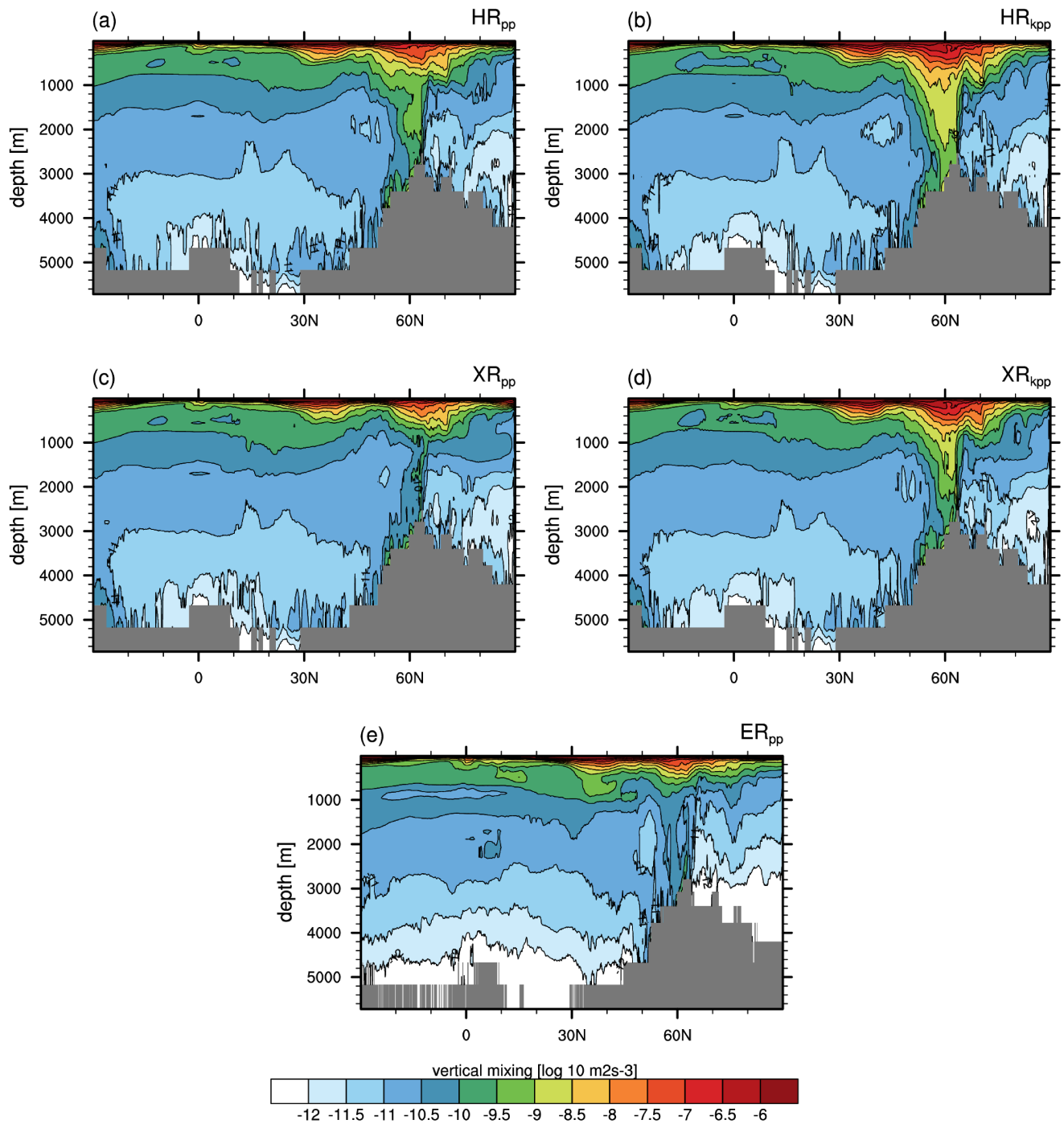
Figure A3. Transect of zonal mean vertical mixing ( \log_{10}(k_v N^2) ) through the Atlantic basin and the Arctic Ocean of (a) \text{HR}_{pp} , (b) \text{HR}_{kpp} , (c) \text{XR}_{pp} , (d) \text{XR}_{kpp} , and (e) \text{ER}_{pp} .
