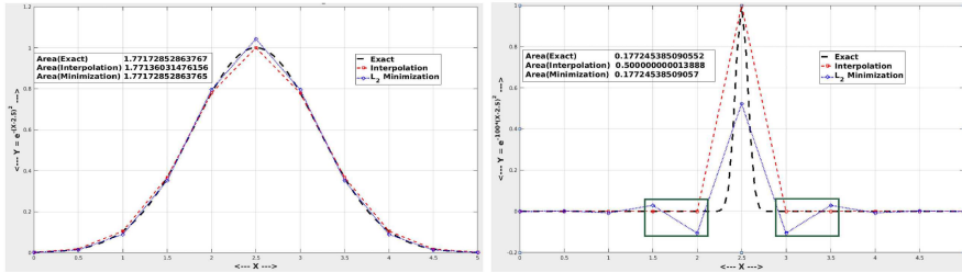
(a) Gaussian hill (x_0, \delta) = (2.5, 1.0)
