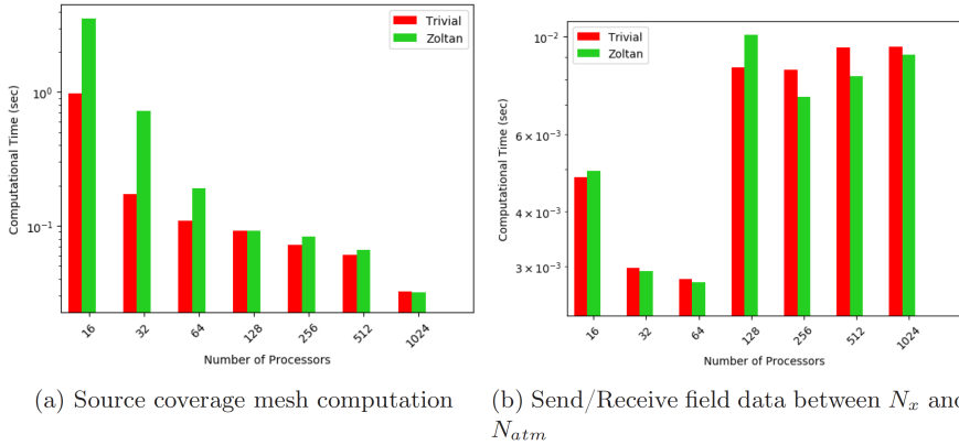
Figure 13. Scaling of the communication kernels driven with the parallel graph computed with a trivial redistribution and the Zoltan geometric (RCB) repartitioner for the NE120 case with N_{ocn} = N_x and N_{atm} = N_x/2 on Cori
