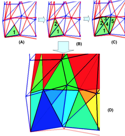
Figure 6. Illustration of the advancing front intersection algorithm.
