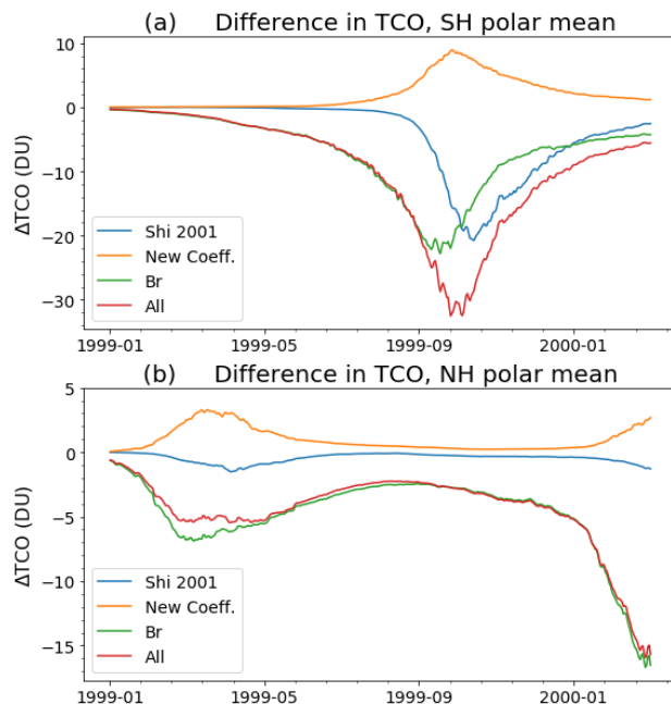
Figure 4. The difference in mean total column ozone (a) south of 65^{\circ}\text{S} and (b) north of 65^{\circ}\text{N} , between the various sensitivity runs and the control run.
