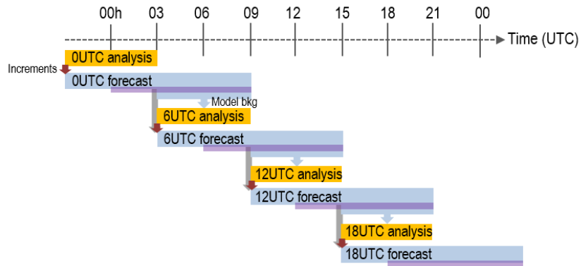
5 Figure 2 Cycling setup of BARRA-R at base time t_0 = 0, 6, 12, and 18 UTC. Each UM forecast is initialized at t_0 - 3h by the previous forecast (grey arrows) with increments from current analysis (red arrows). The purple bars indicate the time steps of the model states that have been archived.
