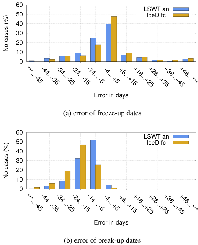
Figure 5. Frequency distribution of the difference between analysed/forecast and observed freeze-up and break-up dates over all lakes 2012-2018. Variables used in diagnosis of ice existence: analysed LSWT crossing the freezing point (blue) and forecast ice thickness > 1 mm (magenta/yellow). Observed variable: freeze-up date by SYKE. x-axis: difference (fc-ob), unit day, y-axis: percentage of all cases.
