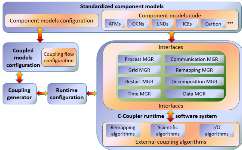
Figure 1 Original software design of C-Coupler (from Liu et al., 2014).
