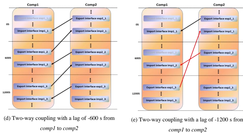
Figure 7 Sample two-way couplings with different lag settings. A coupling interface with light grey words means that it will not be executed, because it corresponds to the coupling interface executed at the model time earlier than the start time (0 s) of the model run
