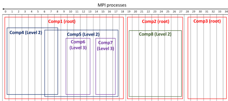
Figure 5 Sample process layout of component models (comp1-comp8).
