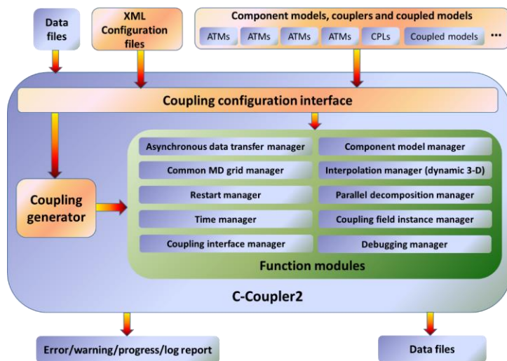
Figure 4 C-Coupler2 software structure.
