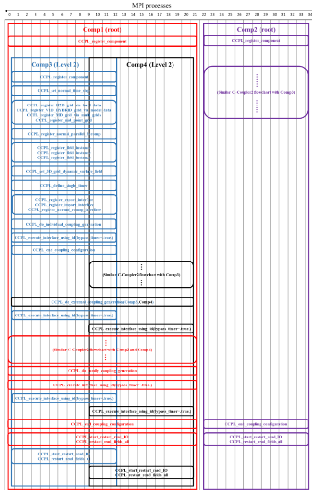
Figure 6—An example of hybrid coupling configuration and model coupling in the initialization stage of a coupled model constructed with C-Coupler2. Comp1–comp4 are the four component models. Labels and boxes of the same color correspond to the same component model.
