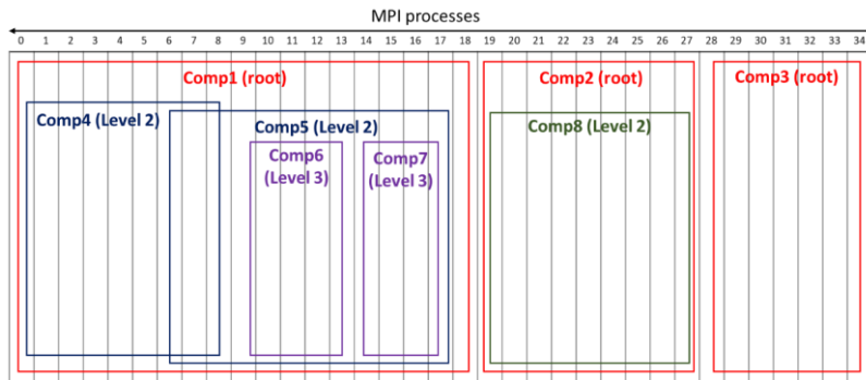
Figure 5 Sample process layout of component models (comp1–comp8).
