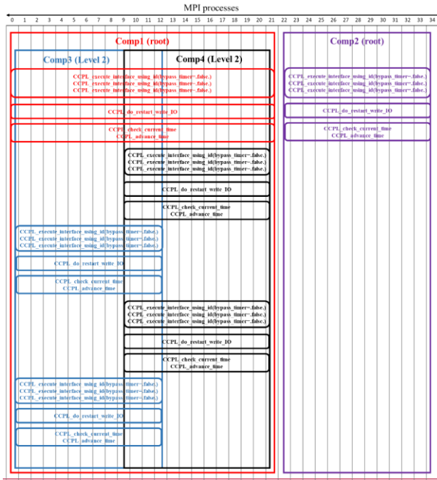
Figure 7 An example of model coupling in the kernel (time integration) stage of a coupled model constructed with C-Coupler2. Comp1-comp4 are the four component models. Labels and boxes of the same color correspond to the same component model.
