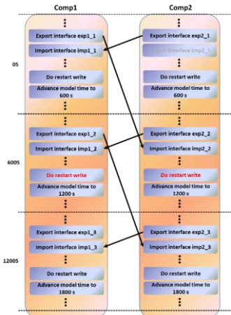
(a) An initial run of a two-way coupled model with a lag of 600 s from comp1 to comp2
