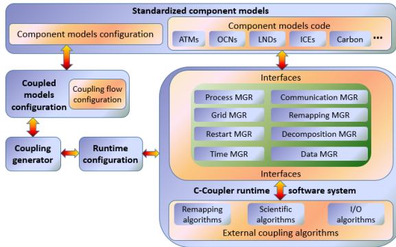
Figure 1 General-Original software designstructure of C-Coupler (from Liu et al., 2014).
