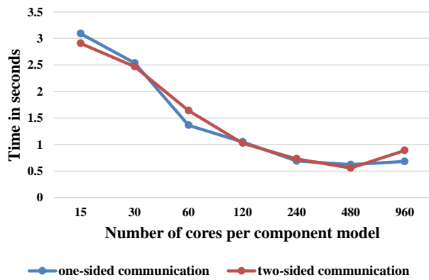
Figure 12 Figure 9 Comparison of data transfer times (for 100 ping-pong couplings) between a one-sided and a two-sided implementation, with the same configuration as Fig. 14 Fig. 8 .
