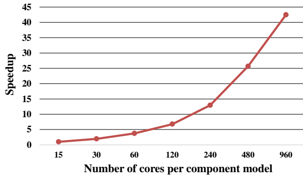
Figure 16 Figure 13 The parallel speedup of dynamic 3-D coupling (for 100 ping-pong couplings) between the two component models, with a new configuration derived from the configuration used in Fig. 14 Fig. 8 . The speedup is normalized to the time at 15 cores per component model (1583 s).
