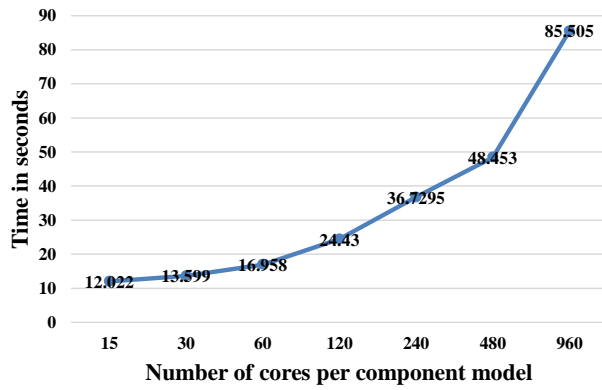
Figure 14 Figure 8 Initialization cost for coupling two toy models with C-Coupler2 on a supercomputer with Intel Xeon CPUs and an InfiniBand network.
