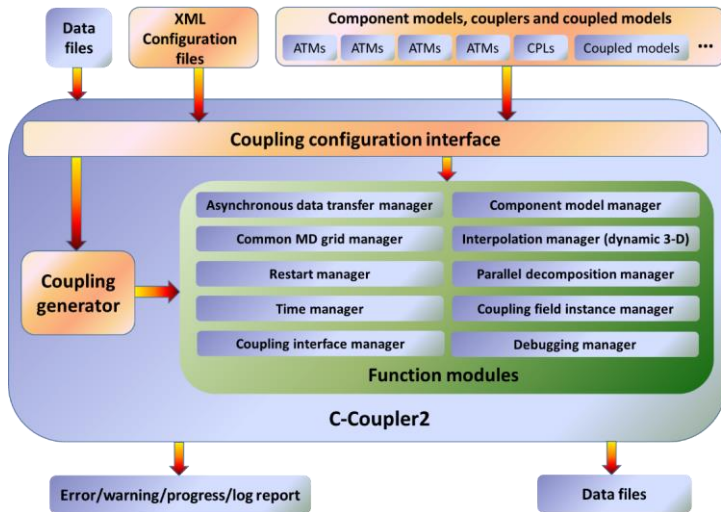
Figure 4 C-Coupler2 software structure.
