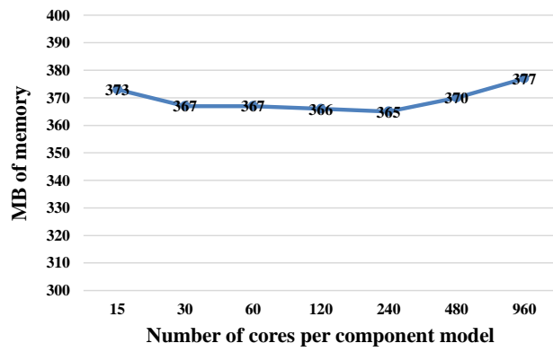
Figure 13 Figure 10 Memory use of C-Coupler2 for the toy coupled model considered in Section 5.2.
