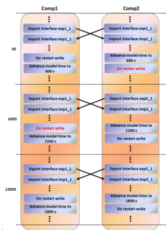
(b) Two-way coupling without lags
