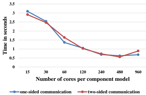
Figure 12 Figure 13 Comparison of data transfer times (for 100 ping-pong couplings) between a one-sided and a two-sided implementation, with the same configuration as Fig. 11 Fig. 12.
