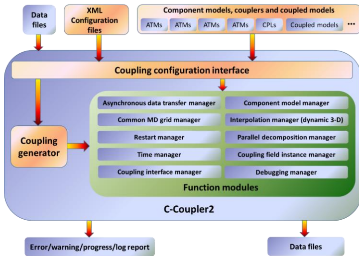
Figure 5 C-Coupler2 software structure.
