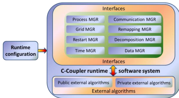
Figure 3 C-Coupler1 software structure.
