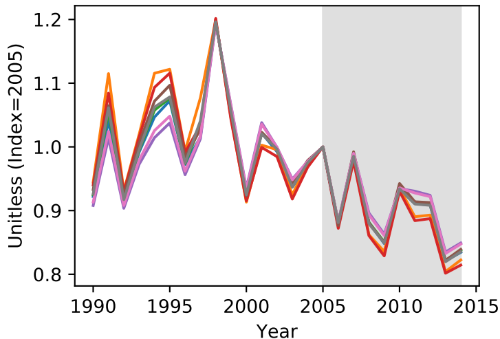
Global Emissions Grass Burning
