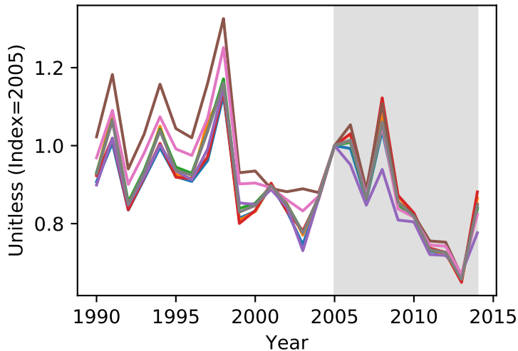
Global Emissions Ag Burning
