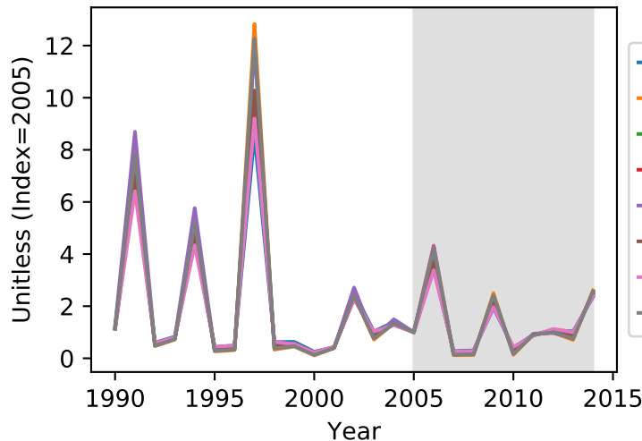
Global Emissions Peat Burning
