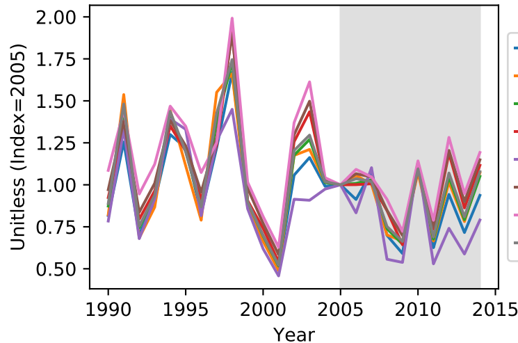
Global Emissions Forest Burning
