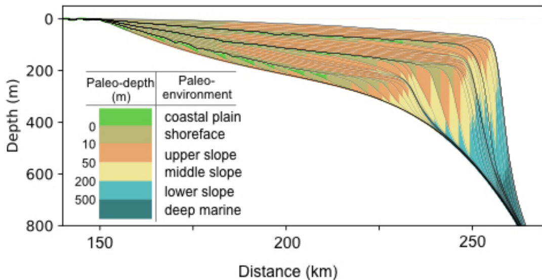
Fig. 3. Supplementar figure to Comment 1_2. Predicted stratal stacking pattern from a new case forced with half of the original subsidence. Other forcing parameters remain the same.
