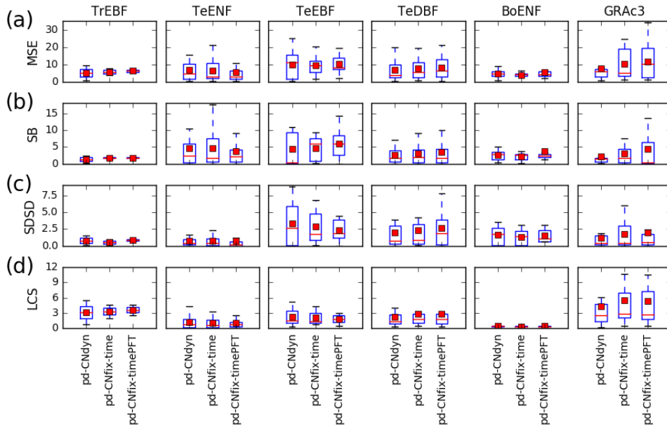
5 Figure 3: Sensitivity of the model performance to the model configuration. Distribution at the plant functional type level of the Mean Square Error (MSE) of the daily GPP variations at each site and contribution to the MSE of model errors on mean value (SB), on standard deviation (SDSD) or on correlation (LCS) for the pd-CNdyn, pd-CNfix-time and pd-CNfix-timepft simulations. The box extends from the lower (25 %) to upper quartile (75 %) values of the data, with a red line at the median and a red square at the arithmetic mean. The whiskers extend from the box to show the range of the data within 1.5 \times (25\text{--}75\%) data range.
