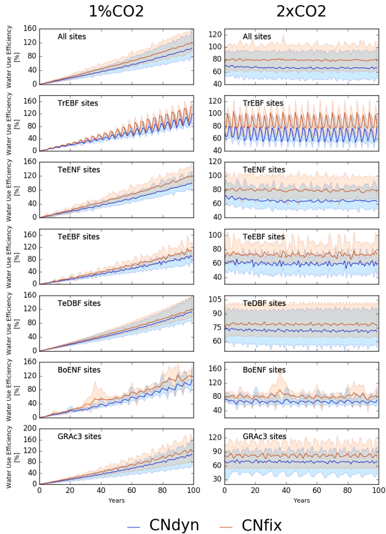
5 Figure 7: Effect of changes in the atmospheric CO 2 concentration on water use efficiency (WUE). Annual mean WUE relative difference [%], mean, 5 and 95 percentile) between the EXP-CNdyn and pd-CNdyn simulations (in blue) and the EXP-CNfix-time and pd-CNfix-time simulations (in red) for the different plant functional types, where EXP stands for 1%CO 2 (left column) and 2xCO 2 (right column). A relative time axis was used because the simulations started the year following the last observational year in the Fluxnet database which may differ across sites.
