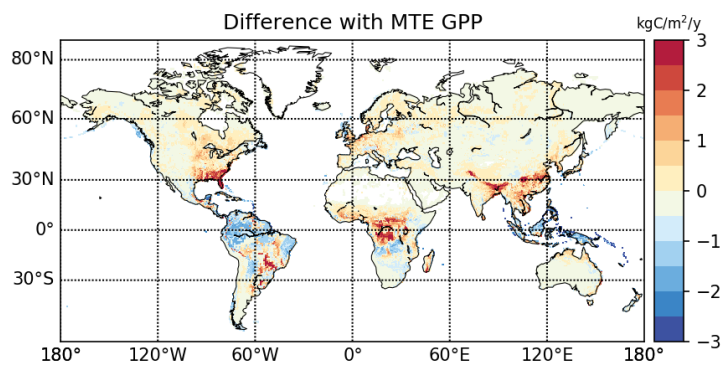
Figure 8: Global scale evaluation of ORCHIDEE r4999 against the observation-based MTE-GPP product. (a) Global distribution of the simulated annual mean GPP ( \text{kgC m}^{-2} \text{yr}^{-1} ) over 2005-2016; (b) Global distribution of the difference between the simulated annual mean GPP and the MTE-GPP product.
