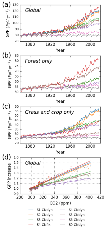
5 Figure 10: Impact of key driving factors on the global annual mean GPP simulated by ORCHIDEE. (A) Simulated global annual mean GPP (PgC yr -1 ) as a function of time, from 1860 to 2016; (B) Simulated annual mean GPP (PgC yr -1 ) of all forest lands from 1860 to 2016; (C) Simulated annual mean GPP (PgC yr -1 ) of all grasslands and croplands from 1860 to 2016; (D) Simulated global annual mean GPP (relatively to its 1900 value) as a function of the [CO 2 ] level. S0-CNdyn to S6-CNdyn are seven additive scenarios where driving factors are added one at a time, and S4-CNfix a scenario where the leaf C/N ratios of each PFT within each grid cell are fixed to their mean-time pre-industrial values (see Sect. 2.4.3 and Table 2 for details). On panel (B), blue, orange and green lines (respectively for S1-CNdyn, S2-CNdyn and S3-CNdyn scenarios) overlay because synthetic fertiliser and manure applications are not considered on forested lands and have consequently no impact on GPP. 10
