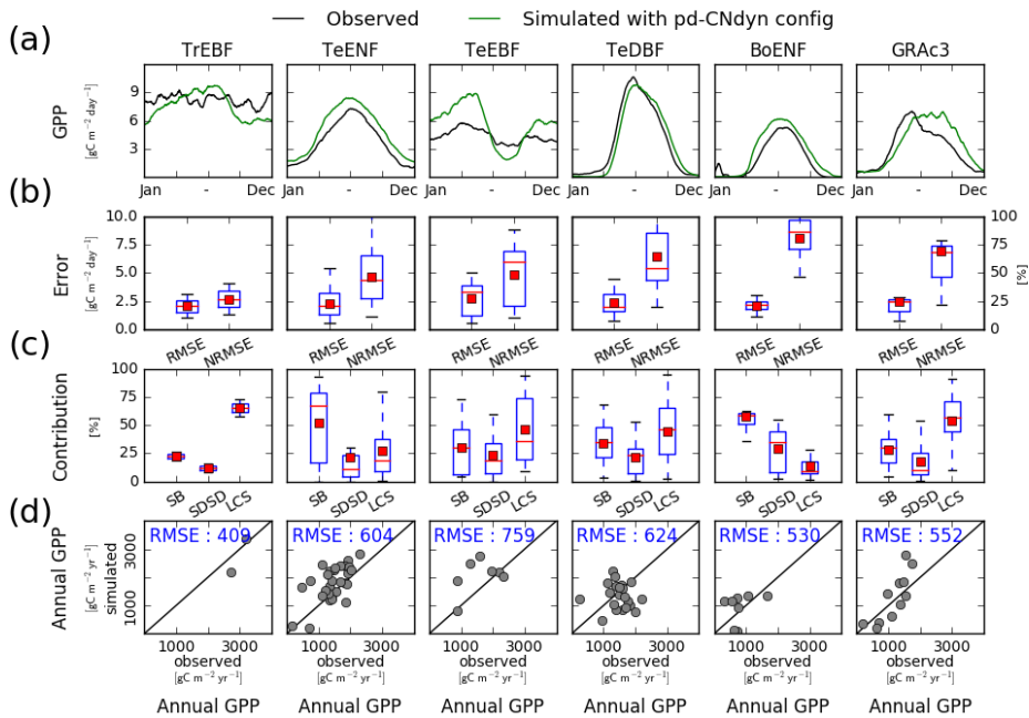
5 Figure 1: Site-level evaluation of ORCHIDEE r4999 simulations against Fluxnet observations. (a) Vegetation-class mean seasonal variations of GPP, (b) Root Mean Square Error (RMSE) and Normalized Root Mean Square Error (NRMSE) of simulated daily variations of GPP per vegetation class, (c) Attribution of the Mean Square Error (MSE) of the daily variations of GPP to model errors on mean value (SB), standard deviation (SDSD) or correlation (LCS) (Kobayashi and Salam, 2000) and (d) simulated vs. observed Annual mean GPP at site-level. On panels (b) and (c), the box extends from the lower (25 %) to upper quartile (75 %) values of the data, with a red line at the median and a red square at the arithmetic mean. The whiskers extend from the box to show the range of the data within 1.5 \times (25-75 \%) data range. 10
