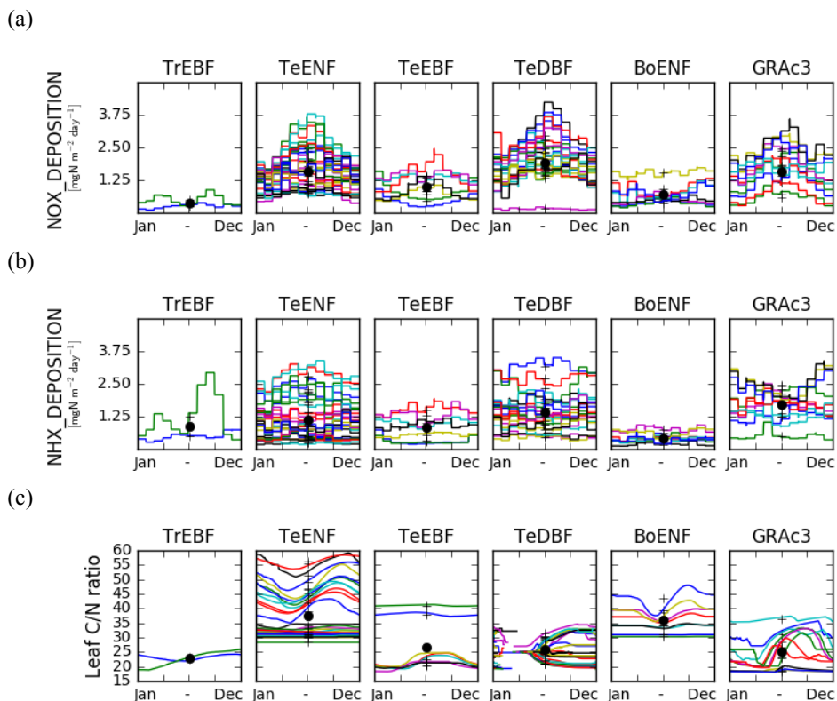
Figure 2: Mean seasonal variations of factors driving the simulated GPP at each site per PFT class. (a) variation of the deposition of NH x compounds, (b) variation of the deposition of NO x compounds and (c) variation of the leaf C/N ratio. Each site is represented by a different colour. The black crosses denote the time-averaged value for each site and the black dots show the time-averaged and site-averaged value for each PFT. Missing data for the leaf C/N ratio of Temperate Deciduous Broadleaved Forests are due to the absence of leaves.
