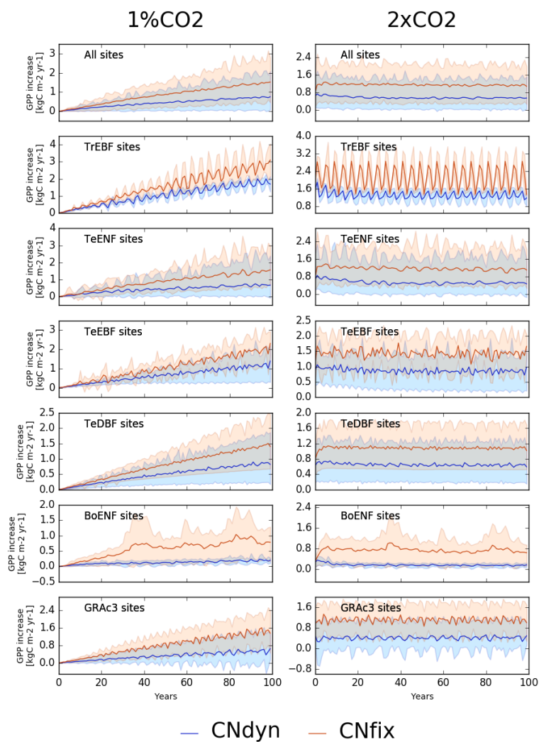
5 Figure 5: Effect of changes in the atmospheric CO 2 concentration on GPP. Annual mean GPP difference (kgC m -2 yr -1 , mean, 5 and 95 percentile) between the EXP-CNdyn and pd-CNdyn simulations (in blue) and the EXP-CNfix-time and pd-CNfix-time simulations (in red) for the different PFTs, where EXP stands for 1%CO 2 (left column) and 2xCO 2 (right column). A relative time axis was used because the simulations started the year following the last observational year in the Fluxnet database which may differ across sites.
