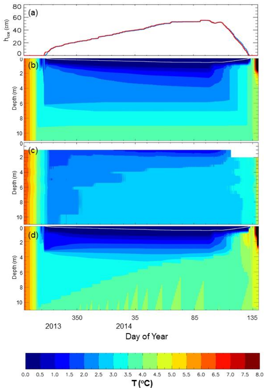
Figure 7: Simulated ice thickness (a), and simulated (b),(d) and observed (c) temperature profiles for 1 November 2013 – 20 May 2014. The standard simulation (MacKay et al. 2017) is shown in (b) and the blue curve in (a). Simulation X2 is shown in (d) and the red curve in (a).
