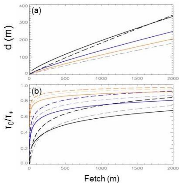
Figure 2: Theoretical IBL depths (a) and surface stress (b) as a function of fetch over water for a rough – to – smooth transition (off shore flow) for forested landscapes (black curves, M=6.9 ); 5 shrubland (blue curves, M=4.6 ), and grassland (red curves, M=2.3 ). Solid curves – Panofsky and Townsend (1964) approach; dashed curves – Jensen (1978) approach with A=1 (thin dashed), and A=2 (thick dashed). Surface stress values are normalized by the theoretical equilibrium downstream value.
