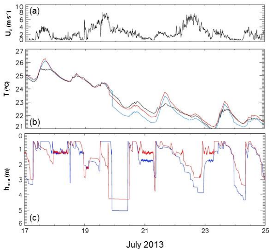
Figure 3: Observed 2-m wind speed (a), observed (black) and simulated 0.5 m water temperatures (b), and simulated diurnal mixed layer depths (c) for 17 – 25 July, 2013. Standard simulation results (blue curves) taken from MacKay et al. (2017). Modified simulation results (red curves) have surface drag coefficient reduced by 50%.
