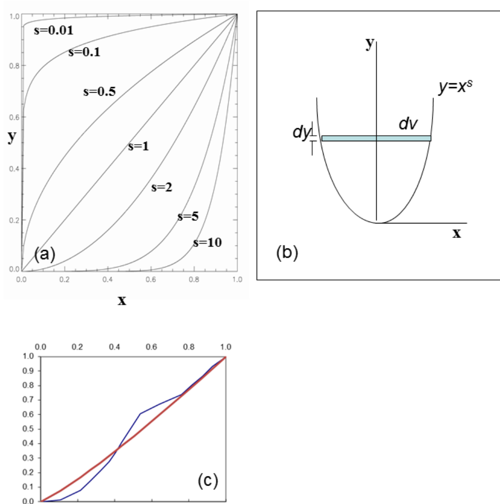
Figure 4: (a) Theoretical “hypsographs” for idealized axially symmetric lakes with different shape factors s indicated; (b) schematic to aid in determining volume of an axially symmetric lake; (c) normalized observed hypsograph (blue) and theoretical estimate (red) for L239. See text for details.
