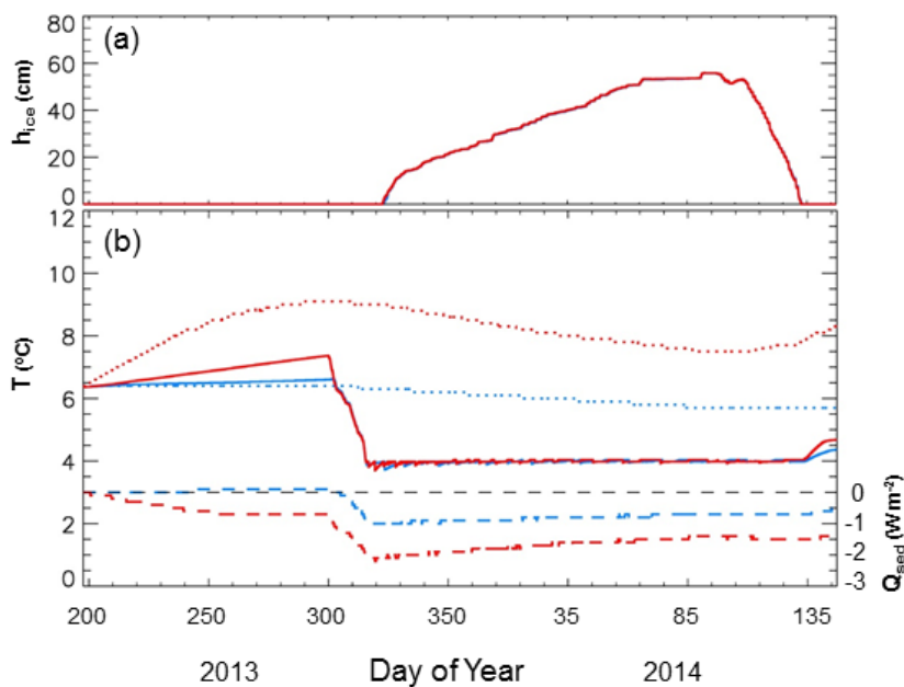
Figure 6: (a) Simulated ice thickness; (b) simulated sediment temperature (dotted), lowest level water temperature (solid), and sediment heat flux (dashed – right hand scale). Simulated results are from experiment X1 (blue) and X2 (red). Zero sediment heat flux (dashed black curve) is also indicated in (b).
