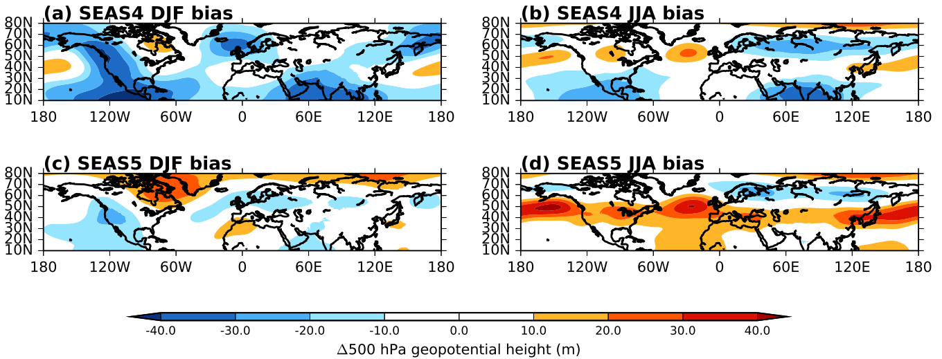
Figure 9. Northern extratropics winter and summer 500 hPa geopotential height bias with respect to ERA-Interim in SEAS4 (a,b) and SEAS5 (c,d) at one month forecast lead.
