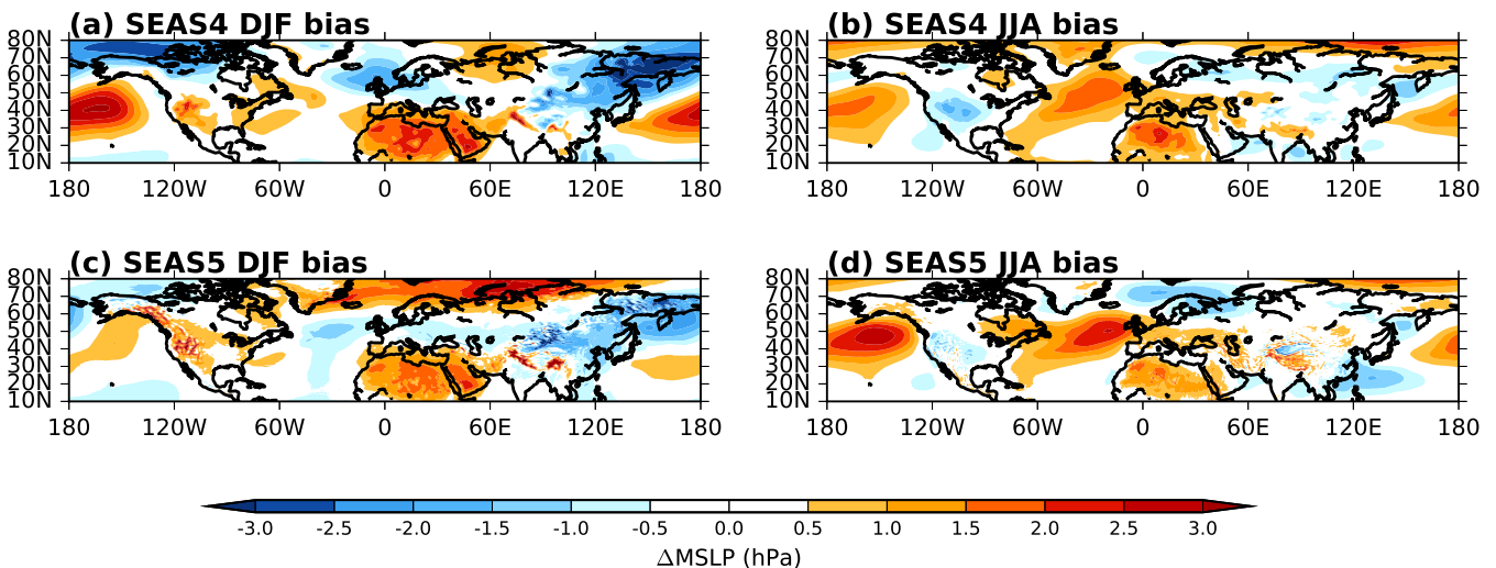
Figure 10. Northern extratropics winter and summer mean sea level pressure bias with respect to ERA-Interim in SEAS4 (a,b) and SEAS5 (c,d) at one month forecast lead.
