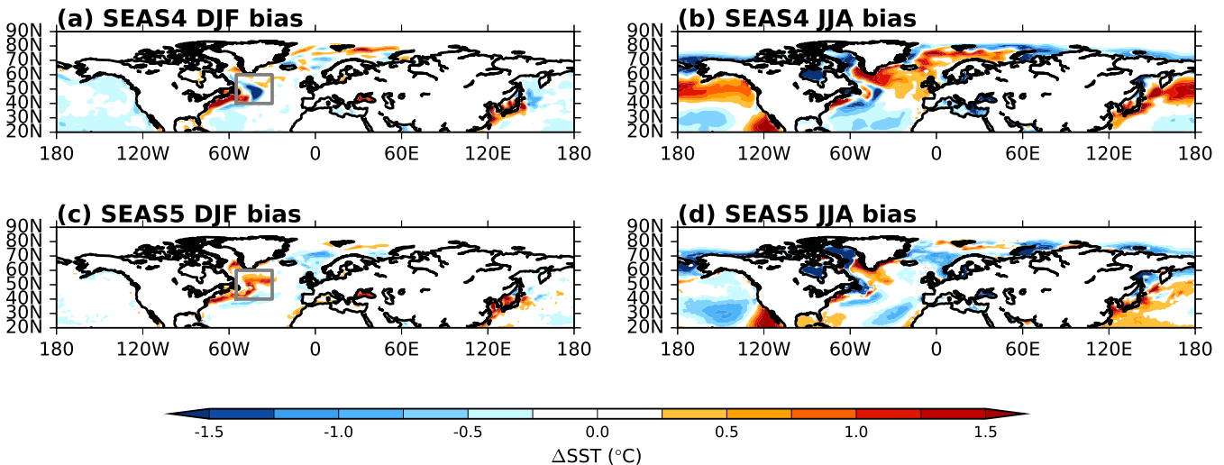
Figure 6. Summer and winter SST bias in the northern extratropics at one month forecast lead for SEAS4 (a,b) and SEAS5 (c,d) compared to the analysis they were initialised from (ORAS4, ORAS5). The region discussed in detail later in this section is outlined in grey here.
