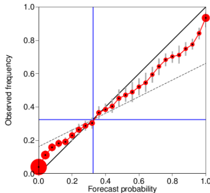
Figure 22. DJF Two-metre temperature reliability diagrams for SEAS5, computed including all grid points for the tropics (left, 20°N to 20°S) and a European region (right, 35° to 75°N, 12.5°W to 42.5°E) over the whole re-forecast period using 25 ensemble members. Verification data is ERA-Interim. Reliability diagrams are computed for three month average forecast anomalies in the upper third of the model climate distribution. Grey vertical lines indicate the 95% confidence intervals.
