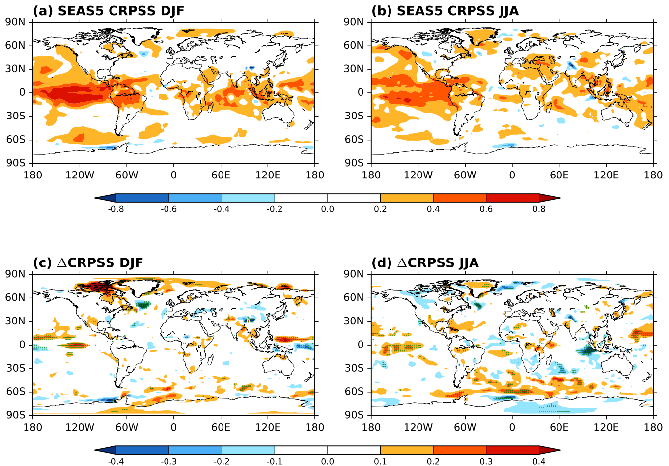
Figure 21. Top: CRPSS maps of two metre temperature skill for SEAS5 with reference to ERA-Interim climatology in (a) DJF and (b) JJA. Bottom: The change in two-metre temperature CRPSS score between SEAS4 and SEAS5 in (c) DJF and (d) JJA. Green stippling is plotted at p < 0.05 .
