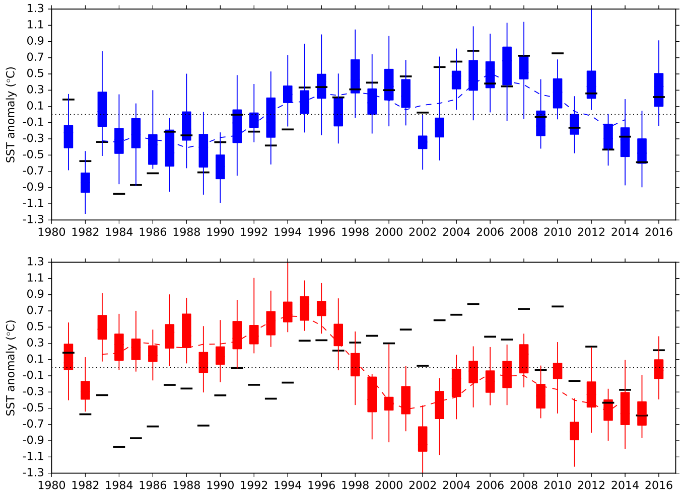
Figure 7. DJF time-series of SST anomaly in a northwest Atlantic region: 50 to 30°W, 40 to 60°N (illustrated as a grey box in Figure 6) at one month forecast lead. Quartiles, minimum and maximum of the SEAS4 25 member ensemble are shown in blue, while the SEAS5 25 member ensemble is shown in red. The black bars indicate ERA-Interim reanalysis. A five-year running mean for each system is shown as a dashed line. Forecasts were initialised in November, and the year shown is the year the ensemble was initialised.
