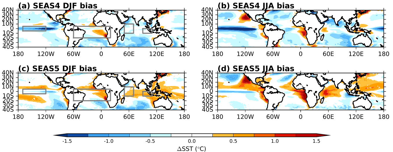
Figure 1. Winter and summer SST bias in the tropics at one month lead forecast for SEAS4 (a,b) and SEAS5 (c,d) compared to the analysis they were initialised from (ORAS4, ORAS5). The regions discussed in detail later in this section are outlined in grey here.
